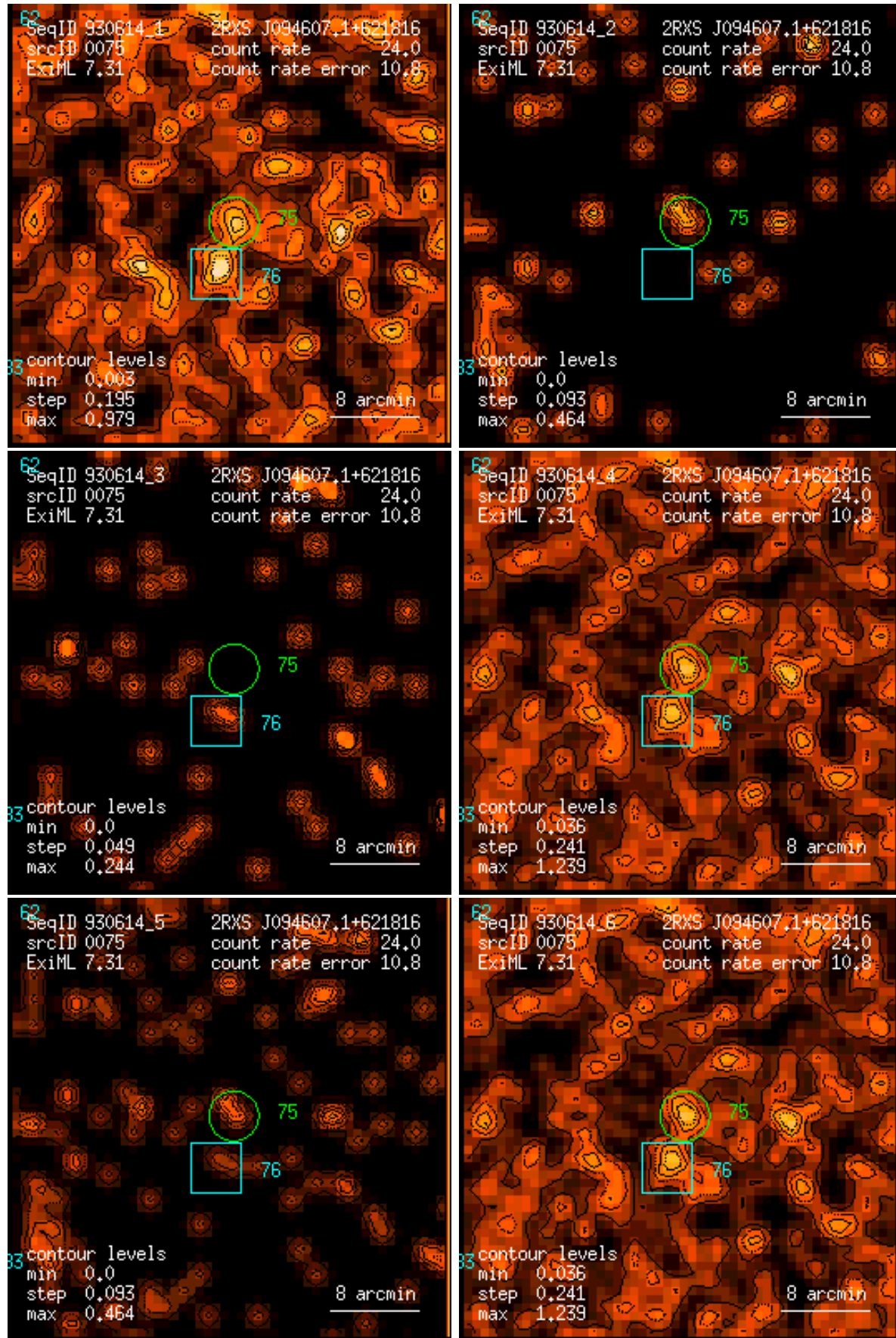
Figure 75: RASS 930614: detection 0075: band rate images, Gaussian filter: (1) PSPC channels 11 – 41, (2) 52 – 90, (3) 91 – 201, (4) 11 – 235, (5) 52 – 201, (6) 11 – 201. Broad band rates in counts/ks. Band rate contour levels in counts/ks/arcmin 2 .
