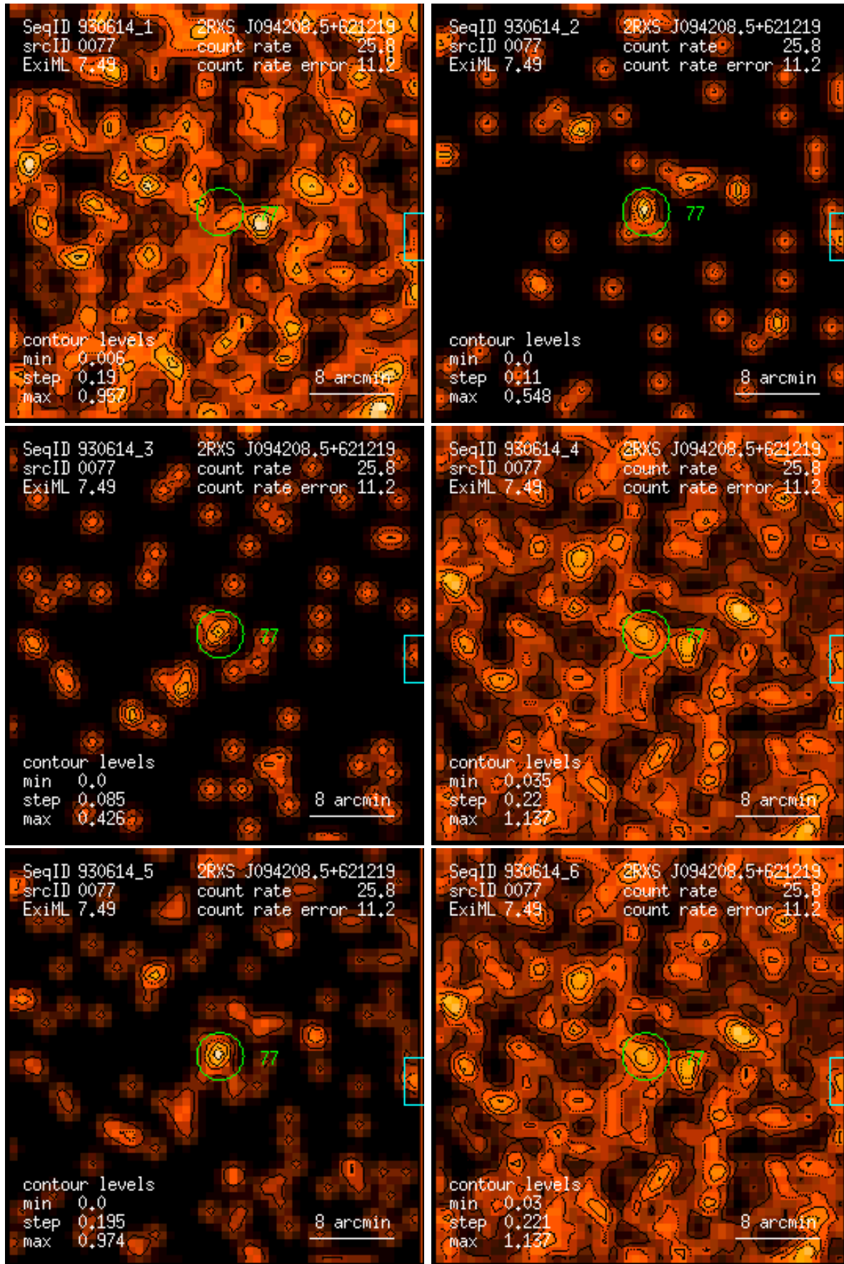
Figure 77: RASS 930614: detection 0077: band rate images, Gaussian filter: (1) PSPC channels 11 – 41, (2) 52 – 90, (3) 91 – 201, (4) 11 – 235, (5) 52 – 201, (6) 11 – 201. Broad band rates in counts/ks. Band rate contour levels in counts/ks/arcmin 2 .
