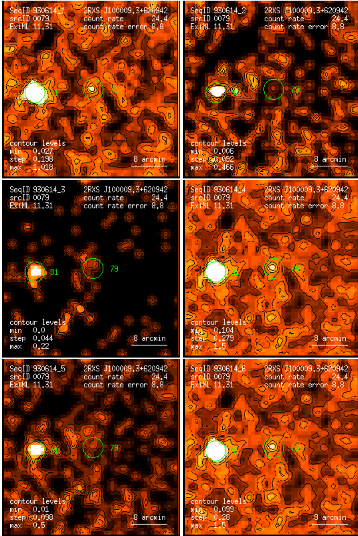
Figure 79: RASS 930614: detection 0079: band rate images, Gaussian filter: (1) PSPC channels 11 – 41, (2) 52 – 90, (3) 91 – 201, (4) 11 – 235, (5) 52 – 201, (6) 11 – 201. Broad band rates in counts/ks. Band rate contour levels in counts/ks/arcmin 2 .
