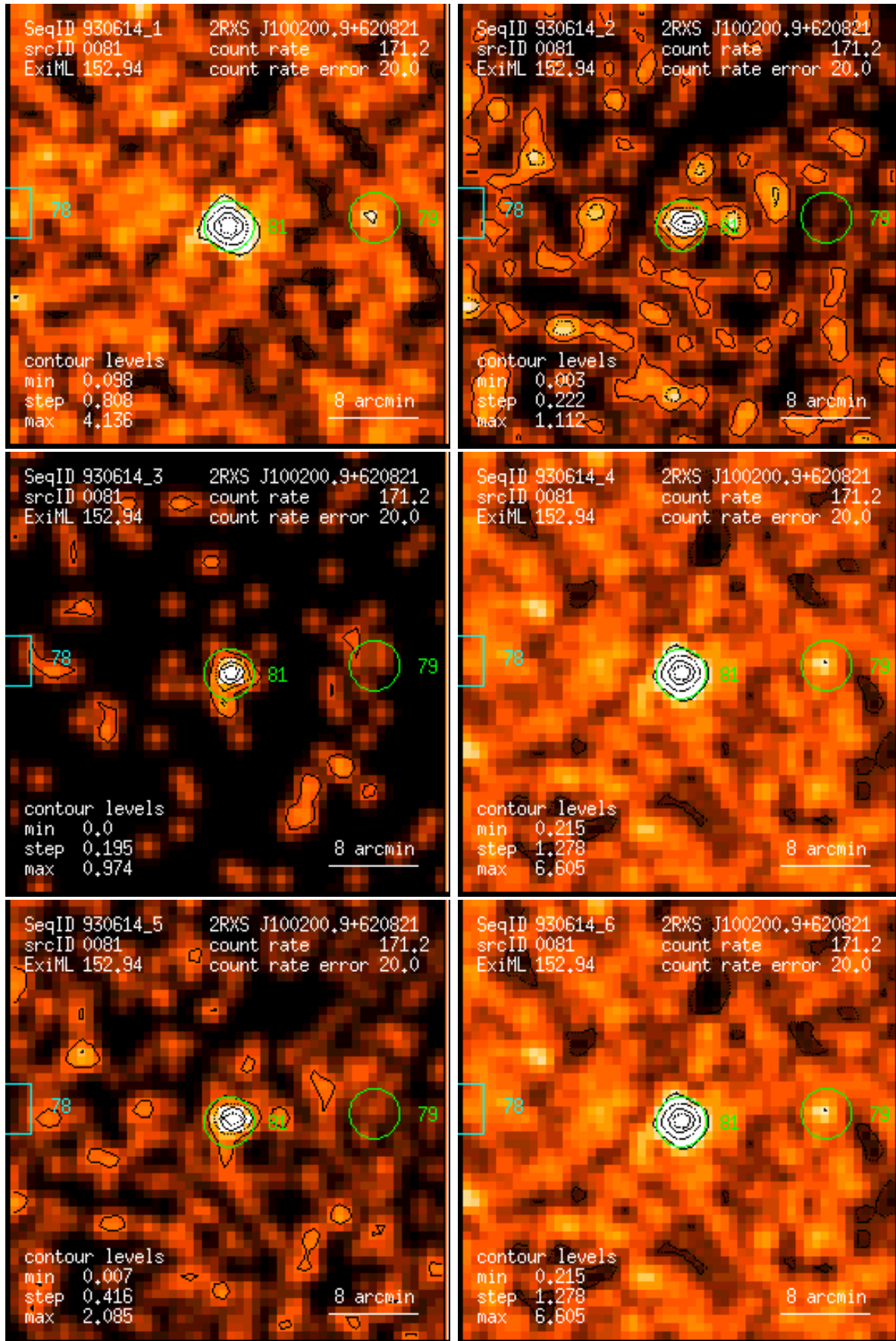
Figure 81: RASS 930614: detection 0081: band rate images, Gaussian filter: (1) PSPC channels 11 – 41, (2) 52 – 90, (3) 91 – 201, (4) 11 – 235, (5) 52 – 201, (6) 11 – 201. Broad band rates in counts/ks. Band rate contour levels in counts/ks/arcmin 2 .
