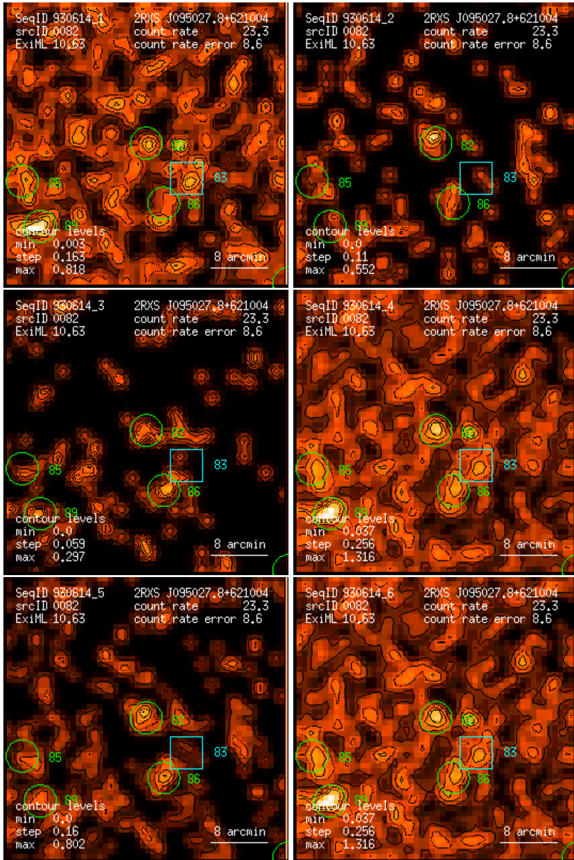
Figure 82: RASS 930614: detection 0082: band rate images, Gaussian filter: (1) PSPC channels 11 – 41, (2) 52 – 90, (3) 91 – 201, (4) 11 – 235, (5) 52 – 201, (6) 11 – 201. Broad band rates in counts/ks. Band rate contour levels in counts/ks/arcmin 2 .
