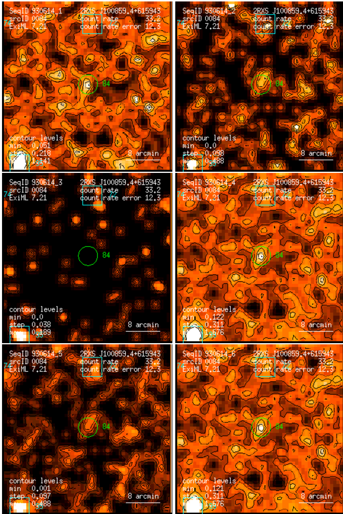
Figure 84: RASS 930614: detection 0084: band rate images, Gaussian filter: (1) PSPC channels 11 – 41, (2) 52 – 90, (3) 91 – 201, (4) 11 – 235, (5) 52 – 201, (6) 11 – 201. Broad band rates in counts/ks. Band rate contour levels in counts/ks/arcmin 2 .
