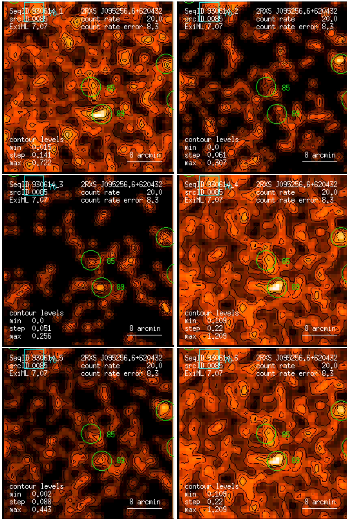
Figure 85: RASS 930614: detection 0085: band rate images, Gaussian filter: (1) PSPC channels 11 – 41, (2) 52 – 90, (3) 91 – 201, (4) 11 – 235, (5) 52 – 201, (6) 11 – 201. Broad band rates in counts/ks. Band rate contour levels in counts/ks/arcmin 2 .
