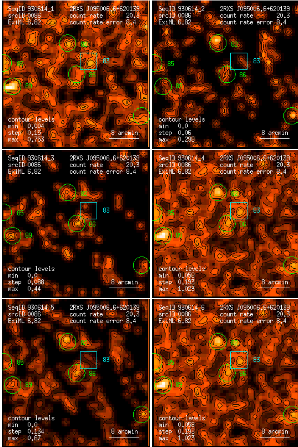
Figure 86: RASS 930614: detection 0086: band rate images, Gaussian filter: (1) PSPC channels 11 – 41, (2) 52 – 90, (3) 91 – 201, (4) 11 – 235, (5) 52 – 201, (6) 11 – 201. Broad band rates in counts/ks. Band rate contour levels in counts/ks/arcmin 2 .
