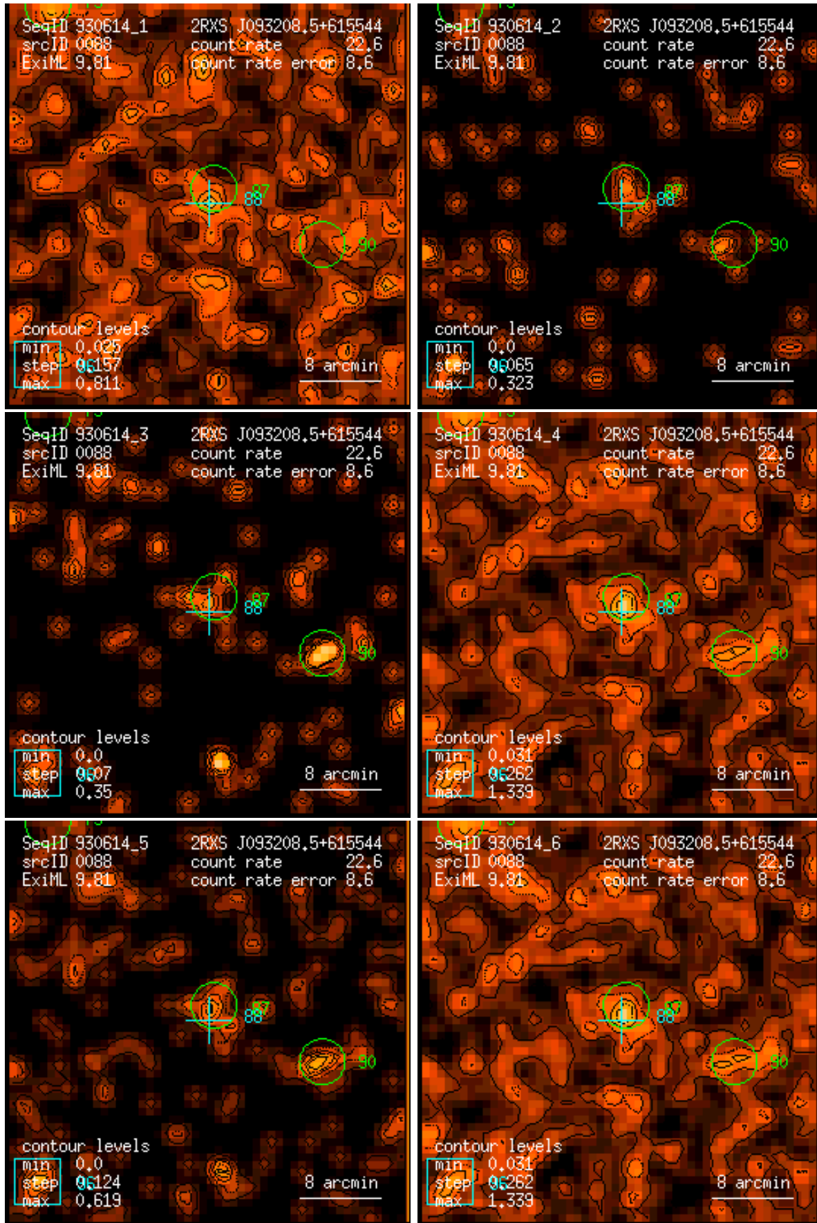
Figure 88: RASS 930614: detection 0088: band rate images, Gaussian filter: (1) PSPC channels 11 – 41, (2) 52 – 90, (3) 91 – 201, (4) 11 – 235, (5) 52 – 201, (6) 11 – 201. Broad band rates in counts/ks. Band rate contour levels in counts/ks/arcmin 2 .
