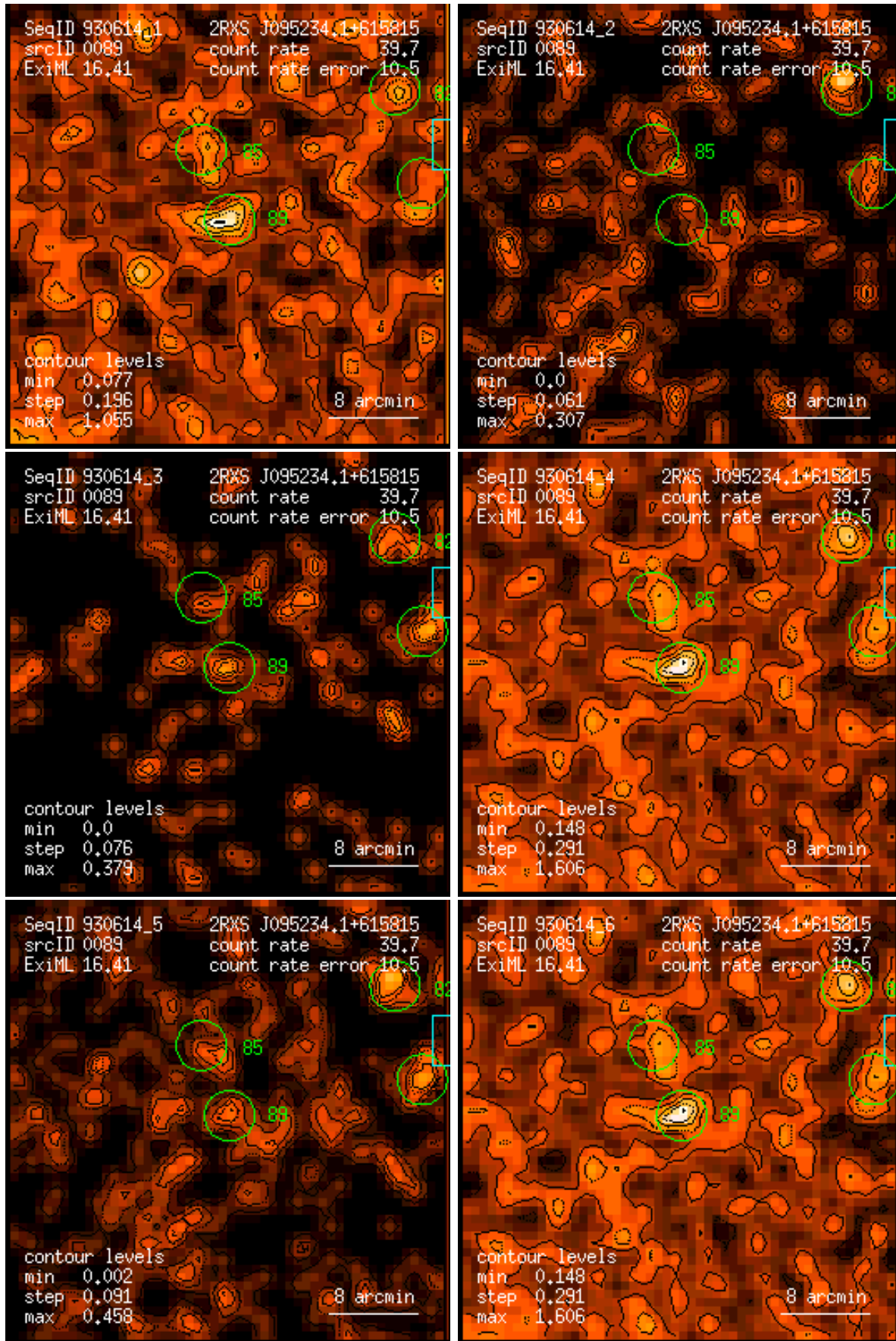
Figure 89: RASS 930614: detection 0089: band rate images, Gaussian filter: (1) PSPC channels 11 – 41, (2) 52 – 90, (3) 91 – 201, (4) 11 – 235, (5) 52 – 201, (6) 11 – 201. Broad band rates in counts/ks. Band rate contour levels in counts/ks/arcmin 2 .
