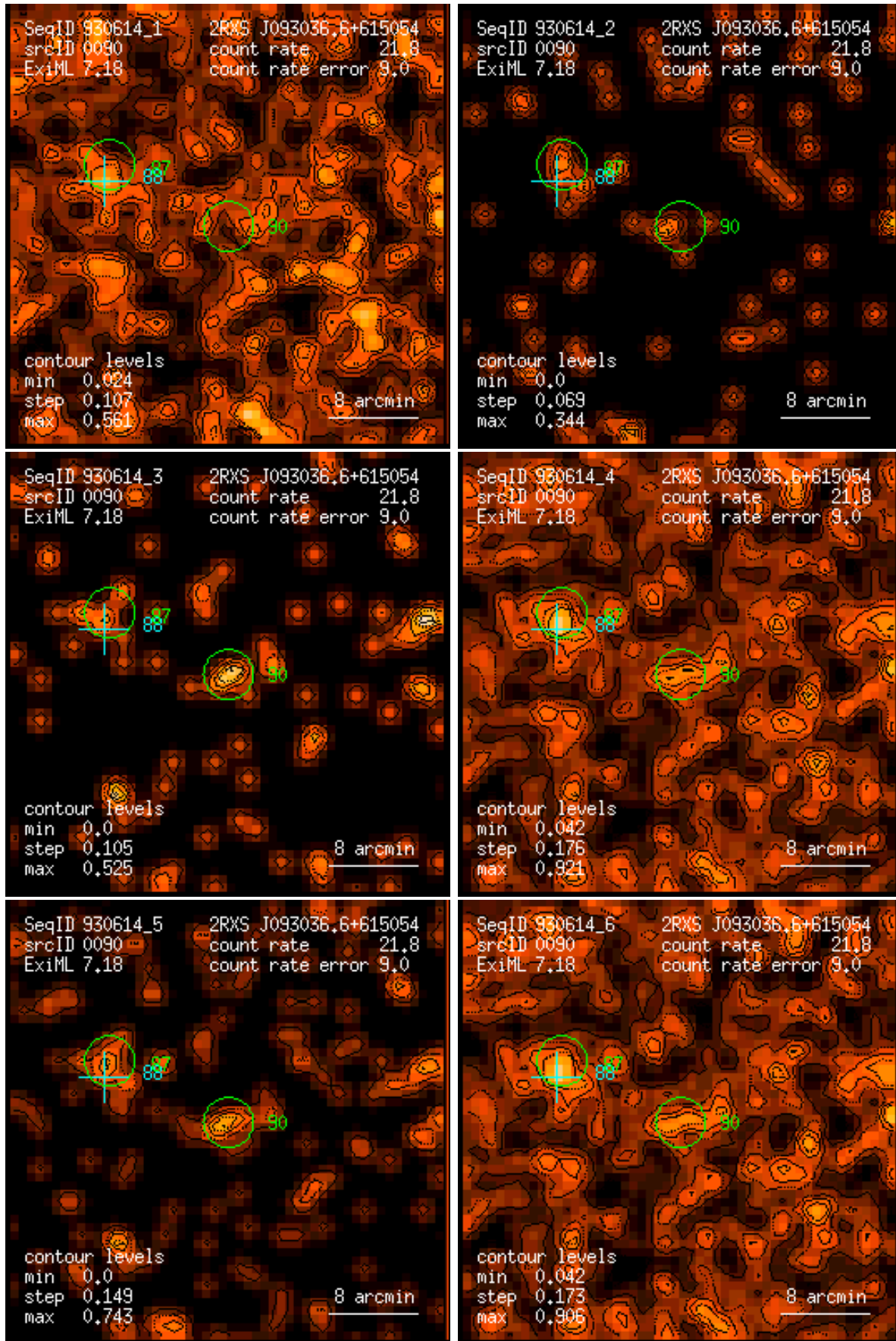
Figure 90: RASS 930614: detection 0090: band rate images, Gaussian filter: (1) PSPC channels 11 – 41, (2) 52 – 90, (3) 91 – 201, (4) 11 – 235, (5) 52 – 201, (6) 11 – 201. Broad band rates in counts/ks. Band rate contour levels in counts/ks/arcmin 2 .
