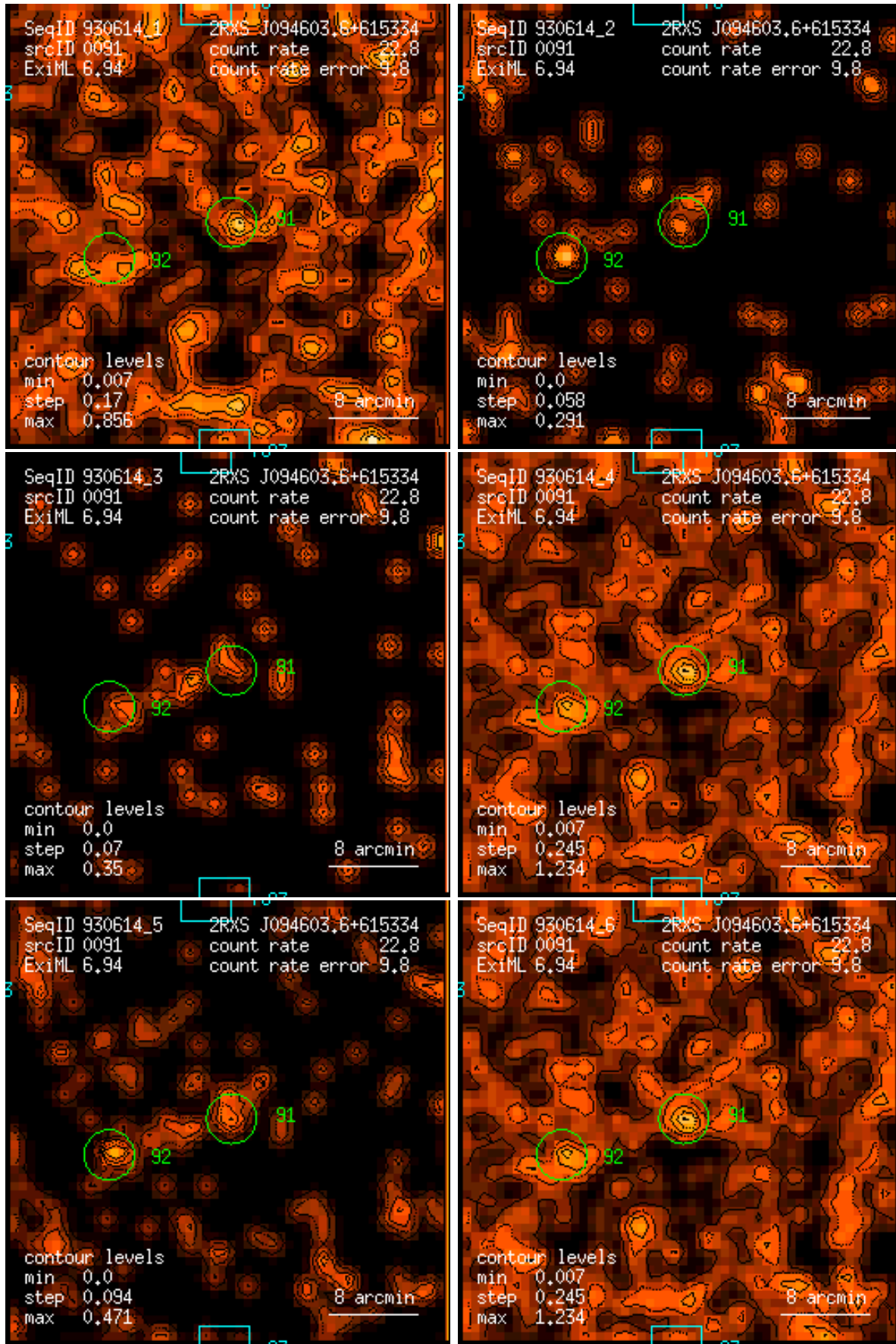
Figure 91: RASS 930614: detection 0091: band rate images, Gaussian filter: (1) PSPC channels 11 – 41, (2) 52 – 90, (3) 91 – 201, (4) 11 – 235, (5) 52 – 201, (6) 11 – 201. Broad band rates in counts/ks. Band rate contour levels in counts/ks/arcmin 2 .
