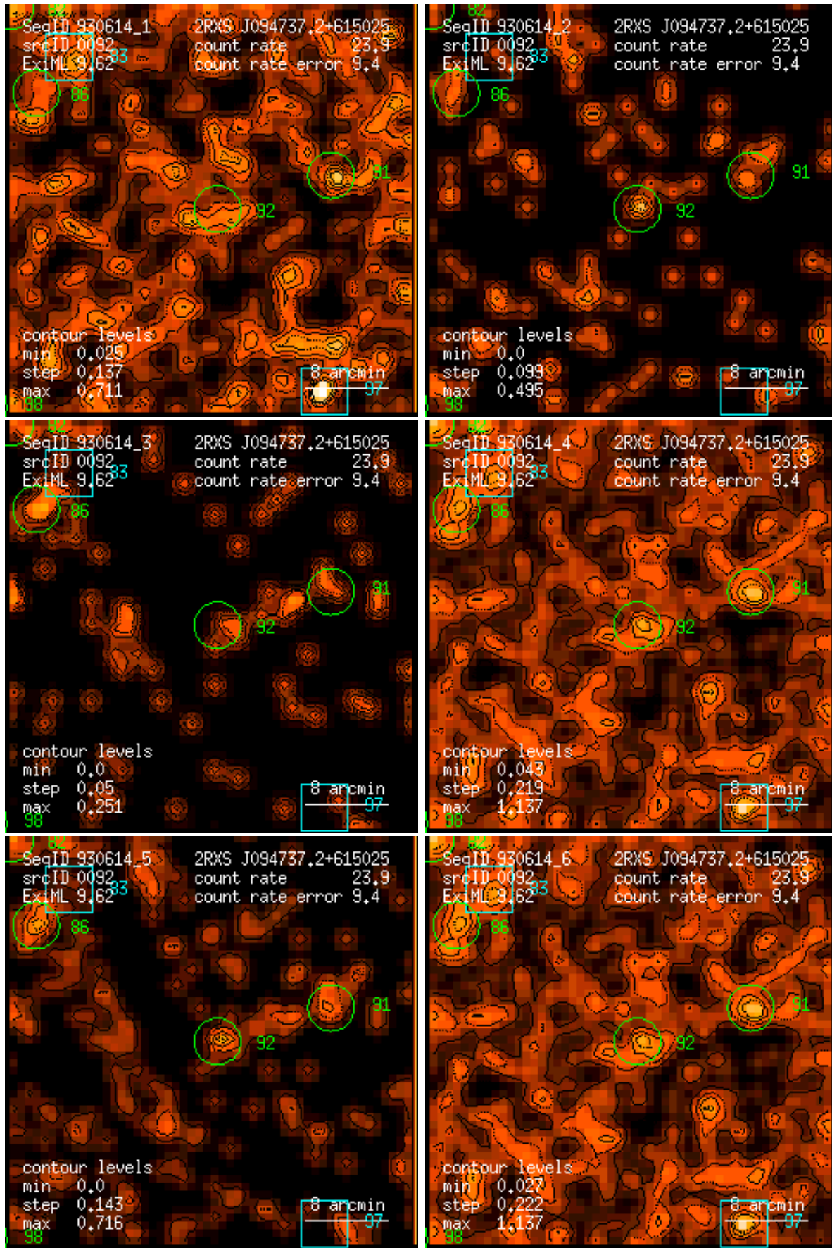
Figure 92: RASS 930614: detection 0092: band rate images, Gaussian filter: (1) PSPC channels 11 – 41, (2) 52 – 90, (3) 91 – 201, (4) 11 – 235, (5) 52 – 201, (6) 11 – 201. Broad band rates in counts/ks. Band rate contour levels in counts/ks/arcmin 2 .
