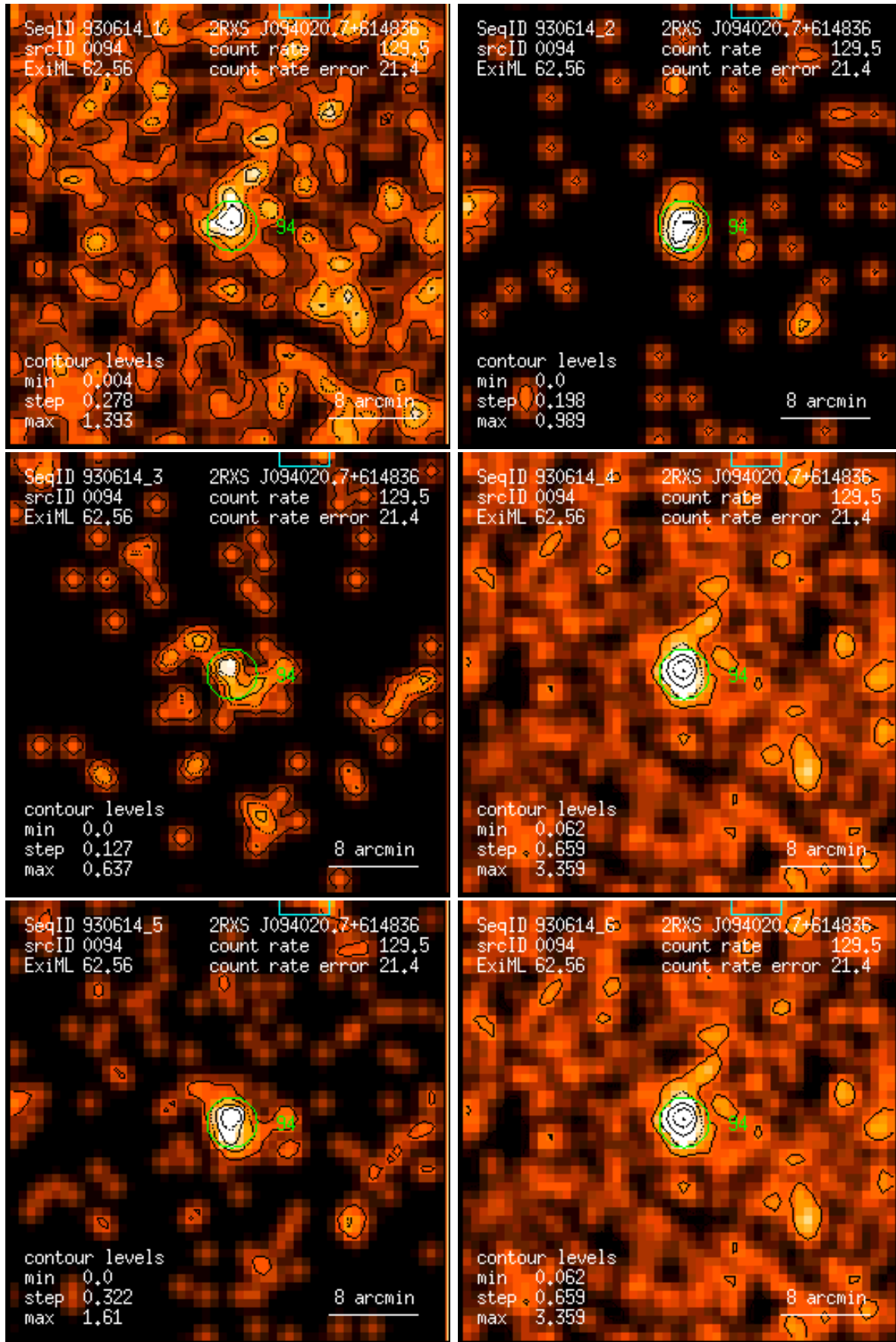
Figure 94: RASS 930614: detection 0094: band rate images, Gaussian filter: (1) PSPC channels 11 – 41, (2) 52 – 90, (3) 91 – 201, (4) 11 – 235, (5) 52 – 201, (6) 11 – 201. Broad band rates in counts/ks. Band rate contour levels in counts/ks/arcmin 2 .
