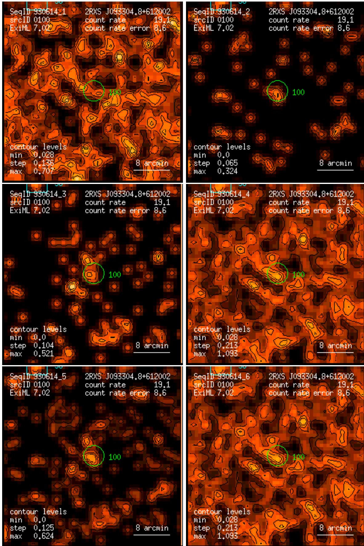
Figure 100: RASS 930614: detection 0100: band rate images, Gaussian filter: (1) PSPC channels 11 – 41, (2) 52 – 90, (3) 91 – 201, (4) 11 – 235, (5) 52 – 201, (6) 11 – 201. Broad band rates in counts/ks. Band rate contour levels in counts/ks/arcmin 2 .
