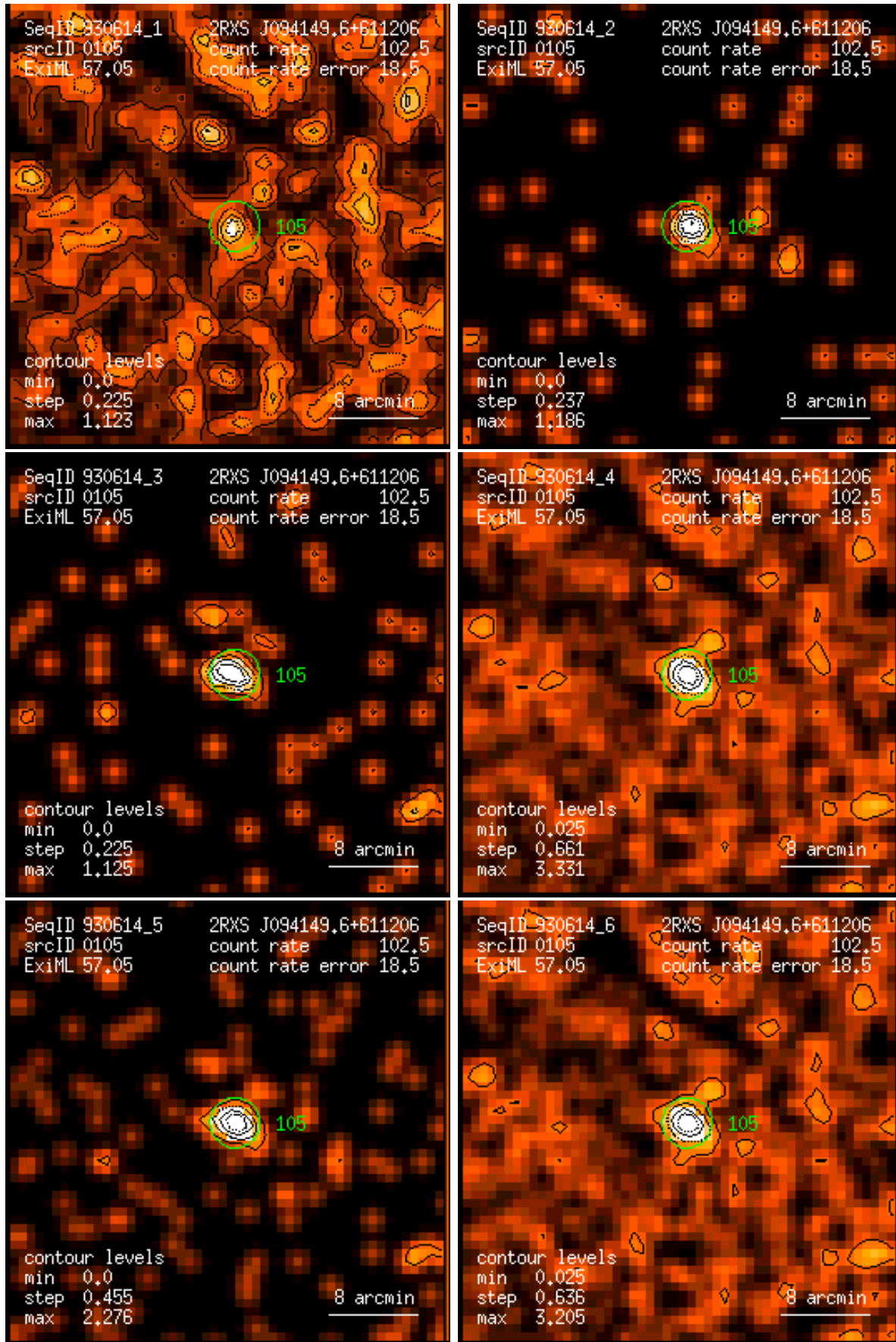
Figure 105: RASS 930614: detection 0105: band rate images, Gaussian filter: (1) PSPC channels 11 – 41, (2) 52 – 90, (3) 91 – 201, (4) 11 – 235, (5) 52 – 201, (6) 11 – 201. Broad band rates in counts/ks. Band rate contour levels in counts/ks/arcmin 2 .
