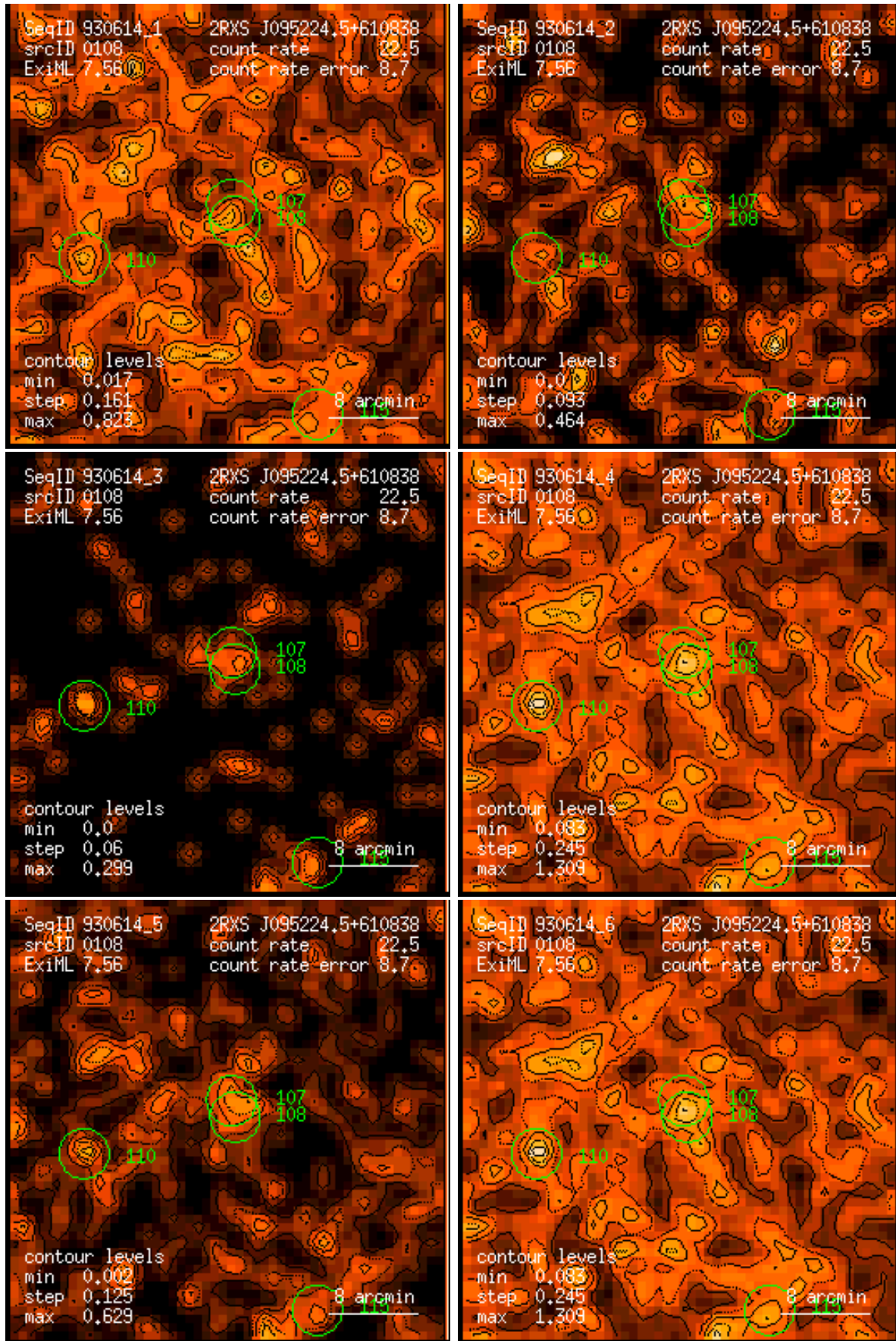
Figure 108: RASS 930614: detection 0108: band rate images, Gaussian filter: (1) PSPC channels 11 – 41, (2) 52 – 90, (3) 91 – 201, (4) 11 – 235, (5) 52 – 201, (6) 11 – 201. Broad band rates in counts/ks. Band rate contour levels in counts/ks/arcmin 2 .
