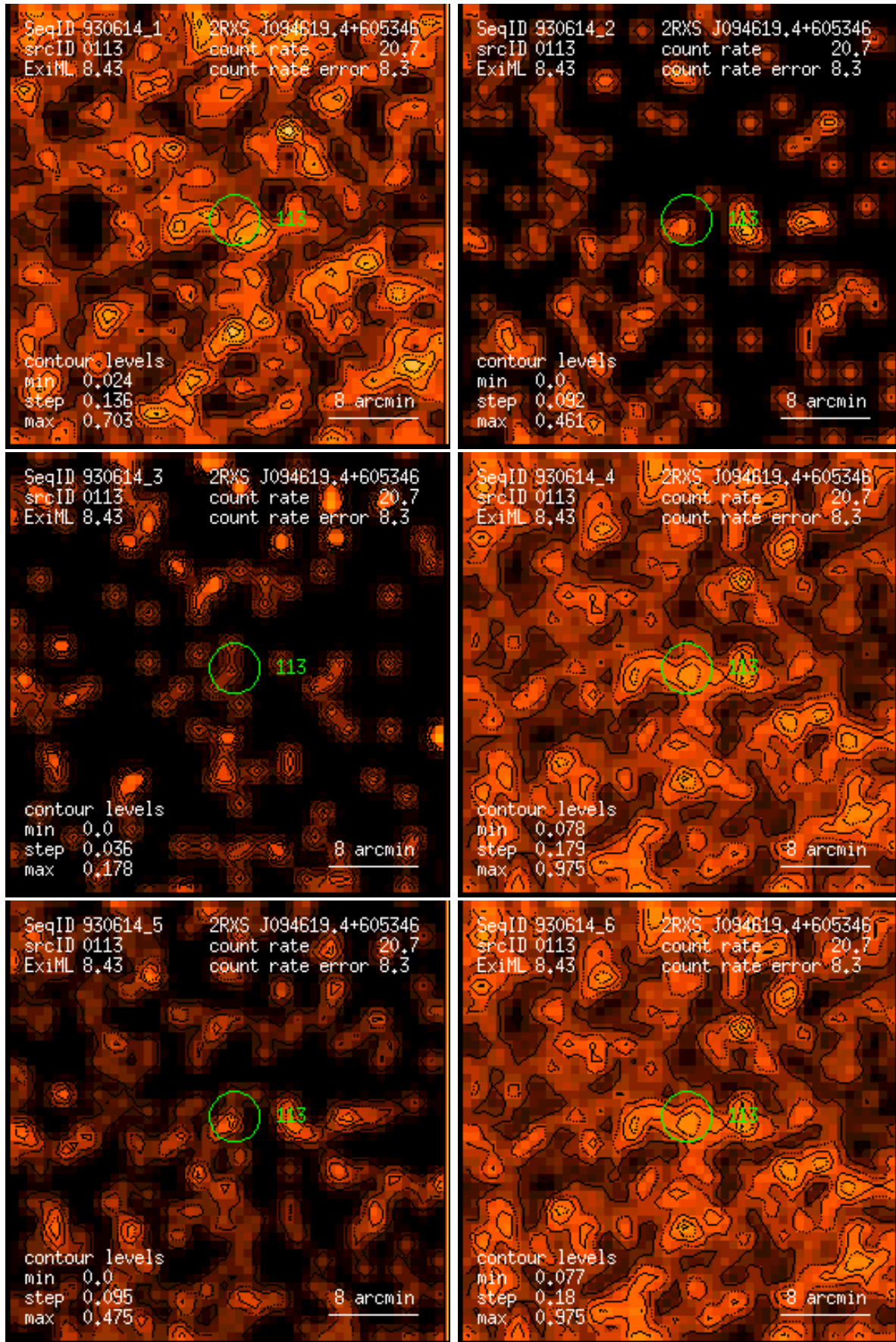
Figure 113: RASS 930614: detection 0113: band rate images, Gaussian filter: (1) PSPC channels 11 – 41, (2) 52 – 90, (3) 91 – 201, (4) 11 – 235, (5) 52 – 201, (6) 11 – 201. Broad band rates in counts/ks. Band rate contour levels in counts/ks/arcmin 2 .
