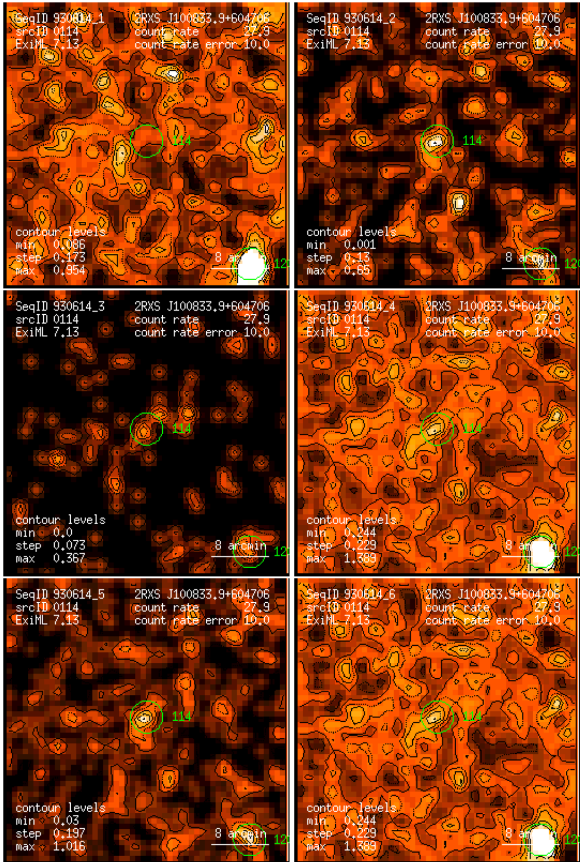
Figure 114: RASS 930614: detection 0114: band rate images, Gaussian filter: (1) PSPC channels 11 – 41, (2) 52 – 90, (3) 91 – 201, (4) 11 – 235, (5) 52 – 201, (6) 11 – 201. Broad band rates in counts/ks. Band rate contour levels in counts/ks/arcmin 2 .
