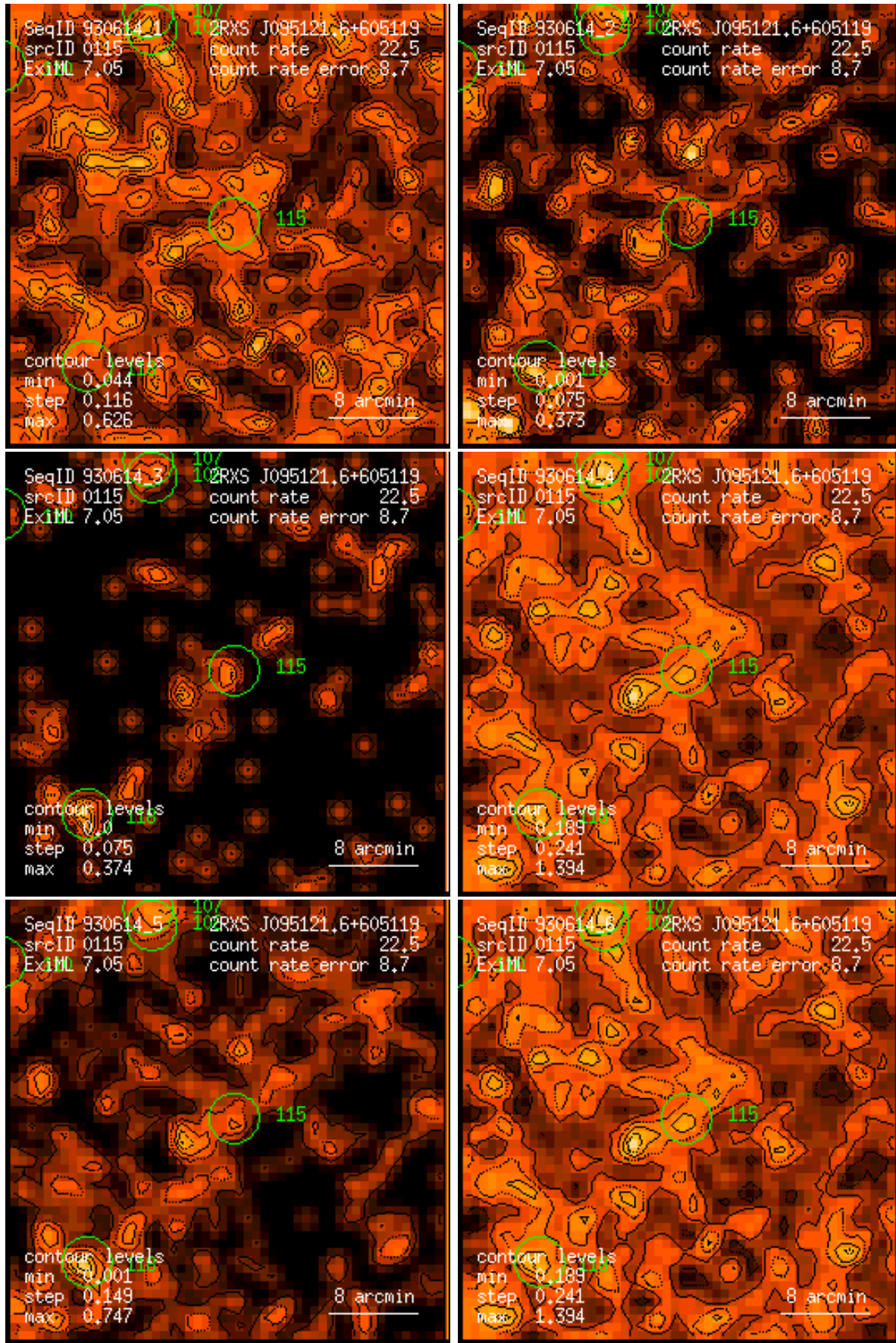
Figure 115: RASS 930614: detection 0115: band rate images, Gaussian filter: (1) PSPC channels 11 – 41, (2) 52 – 90, (3) 91 – 201, (4) 11 – 235, (5) 52 – 201, (6) 11 – 201. Broad band rates in counts/ks. Band rate contour levels in counts/ks/arcmin 2 .
