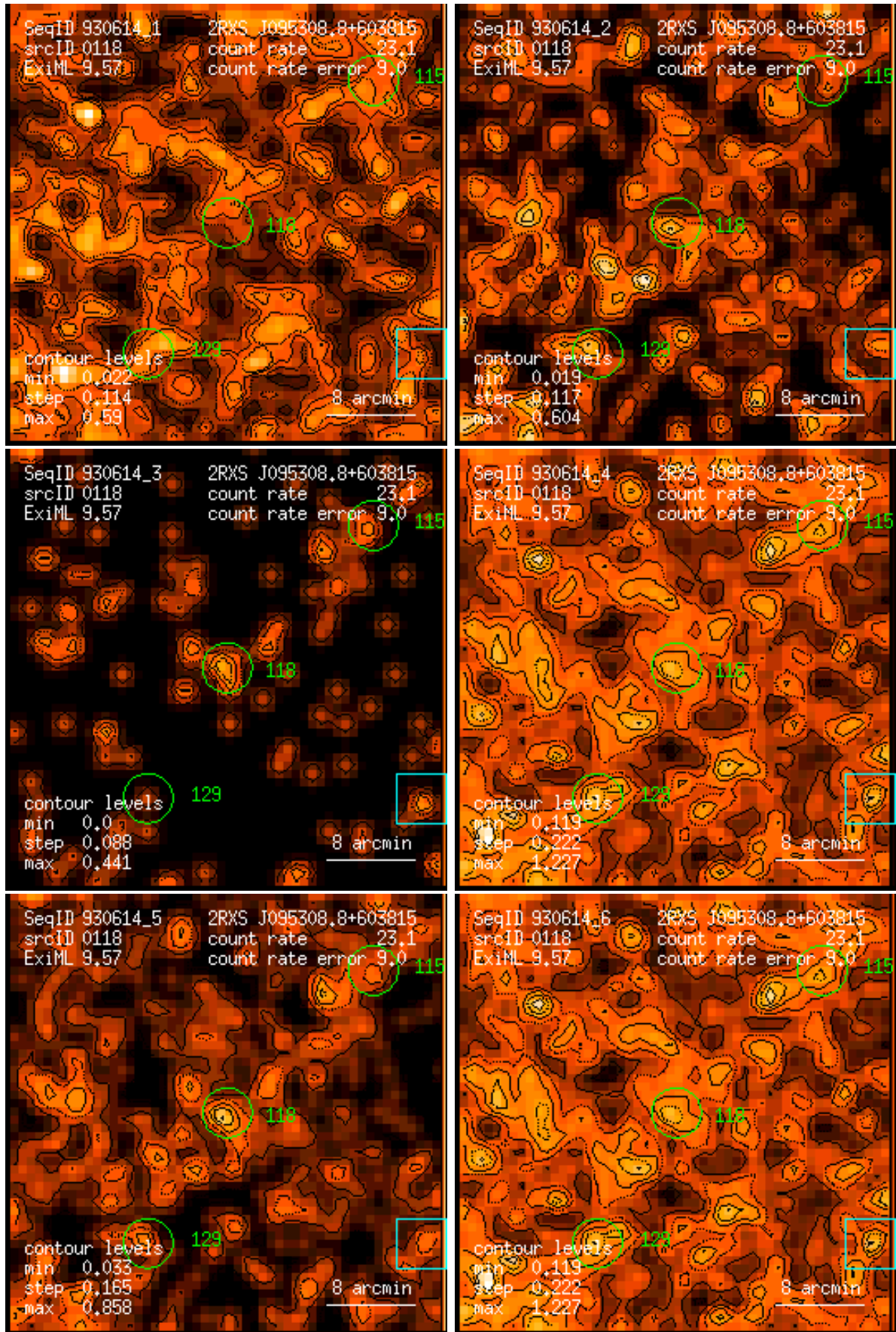
Figure 118: RASS 930614: detection 0118: band rate images, Gaussian filter: (1) PSPC channels 11 – 41, (2) 52 – 90, (3) 91 – 201, (4) 11 – 235, (5) 52 – 201, (6) 11 – 201. Broad band rates in counts/ks. Band rate contour levels in counts/ks/arcmin 2 .
