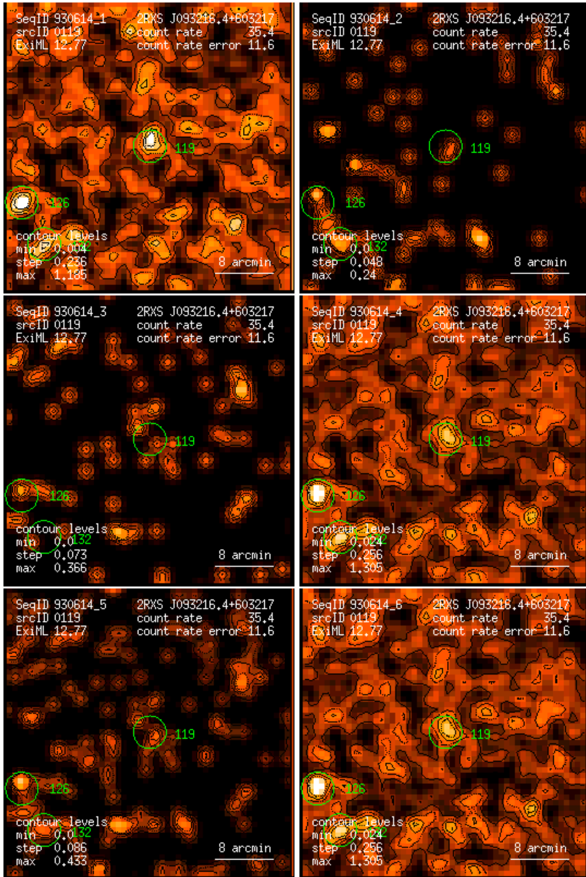
Figure 119: RASS 930614: detection 0119: band rate images, Gaussian filter: (1) PSPC channels 11 – 41, (2) 52 – 90, (3) 91 – 201, (4) 11 – 235, (5) 52 – 201, (6) 11 – 201. Broad band rates in counts/ks. Band rate contour levels in counts/ks/arcmin 2 .
