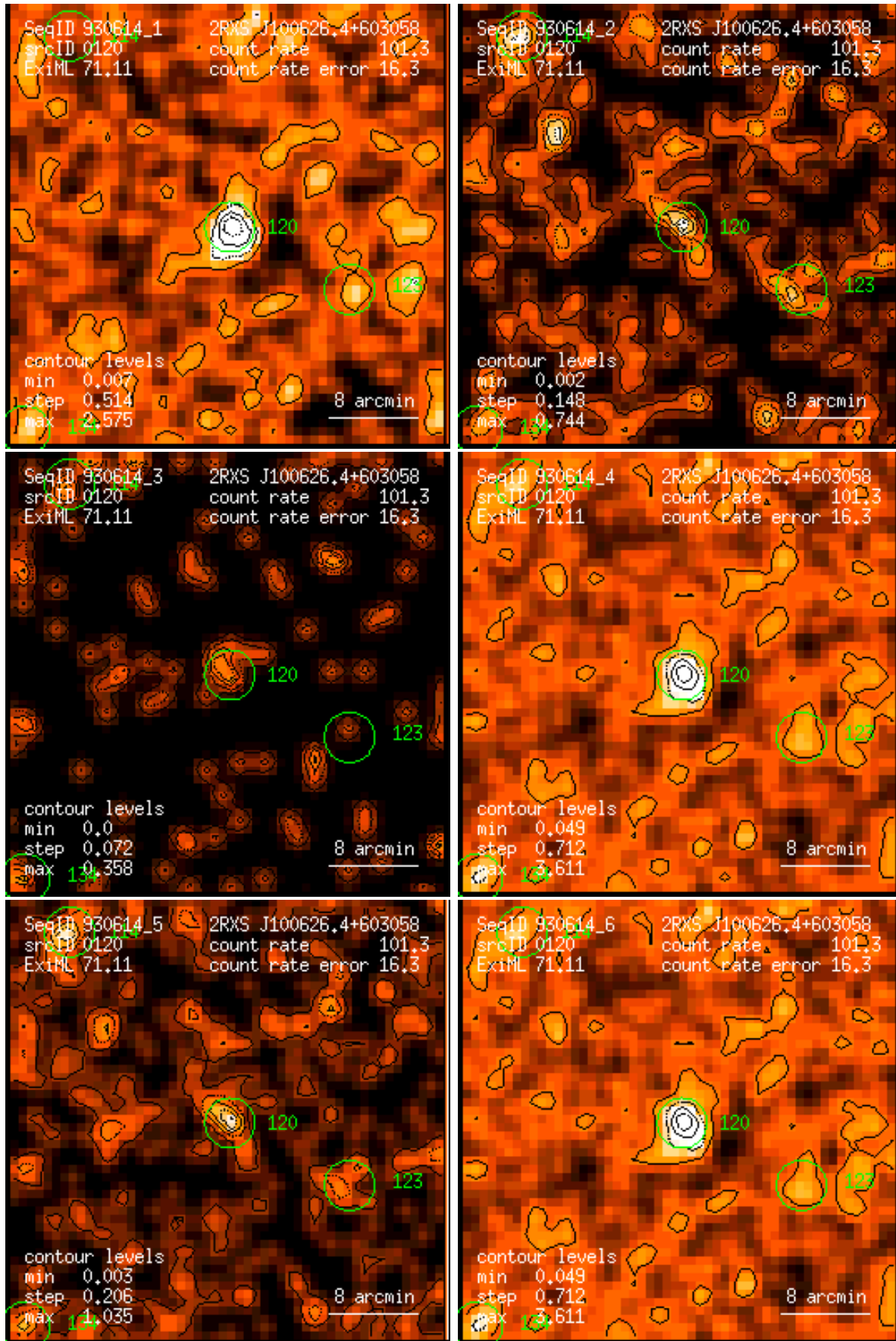
Figure 120: RASS 930614: detection 0120: band rate images, Gaussian filter: (1) PSPC channels 11 – 41, (2) 52 – 90, (3) 91 – 201, (4) 11 – 235, (5) 52 – 201, (6) 11 – 201. Broad band rates in counts/ks. Band rate contour levels in counts/ks/arcmin 2 .
