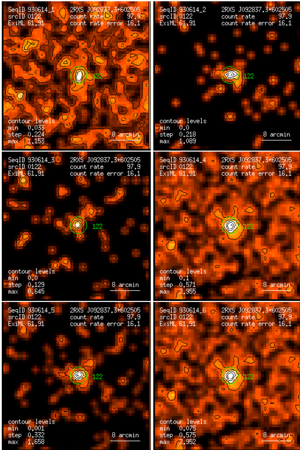
Figure 122: RASS 930614: detection 0122: band rate images, Gaussian filter: (1) PSPC channels 11 – 41, (2) 52 – 90, (3) 91 – 201, (4) 11 – 235, (5) 52 – 201, (6) 11 – 201. Broad band rates in counts/ks. Band rate contour levels in counts/ks/arcmin 2 .
