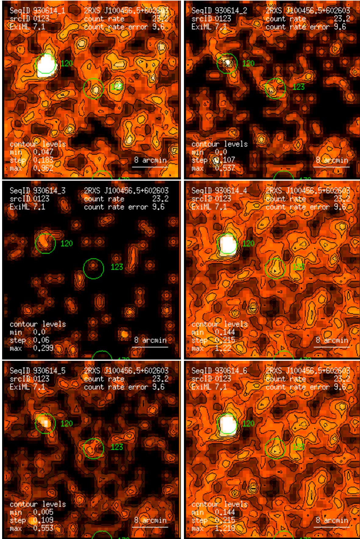
Figure 123: RASS 930614: detection 0123: band rate images, Gaussian filter: (1) PSPC channels 11 – 41, (2) 52 – 90, (3) 91 – 201, (4) 11 – 235, (5) 52 – 201, (6) 11 – 201. Broad band rates in counts/ks. Band rate contour levels in counts/ks/arcmin 2 .
