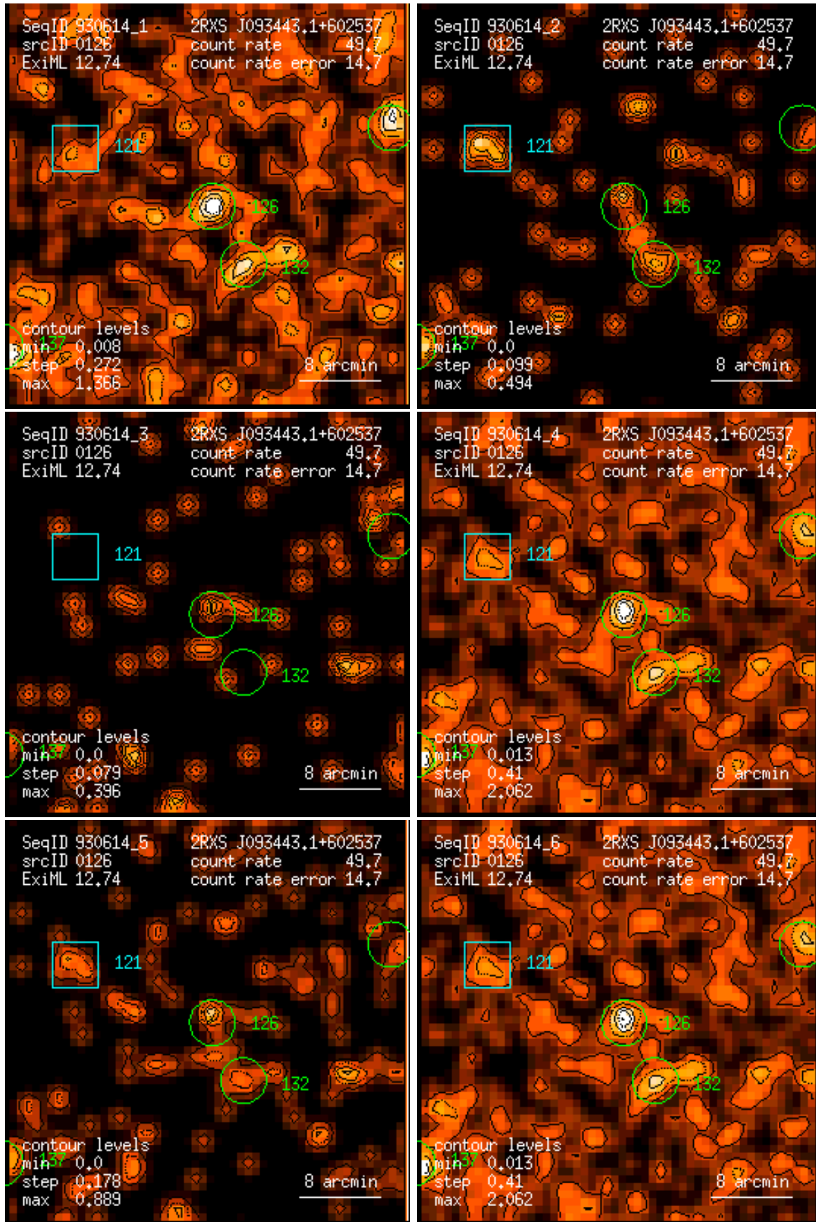
Figure 126: RASS 930614: detection 0126: band rate images, Gaussian filter: (1) PSPC channels 11 – 41, (2) 52 – 90, (3) 91 – 201, (4) 11 – 235, (5) 52 – 201, (6) 11 – 201. Broad band rates in counts/ks. Band rate contour levels in counts/ks/arcmin 2 .
