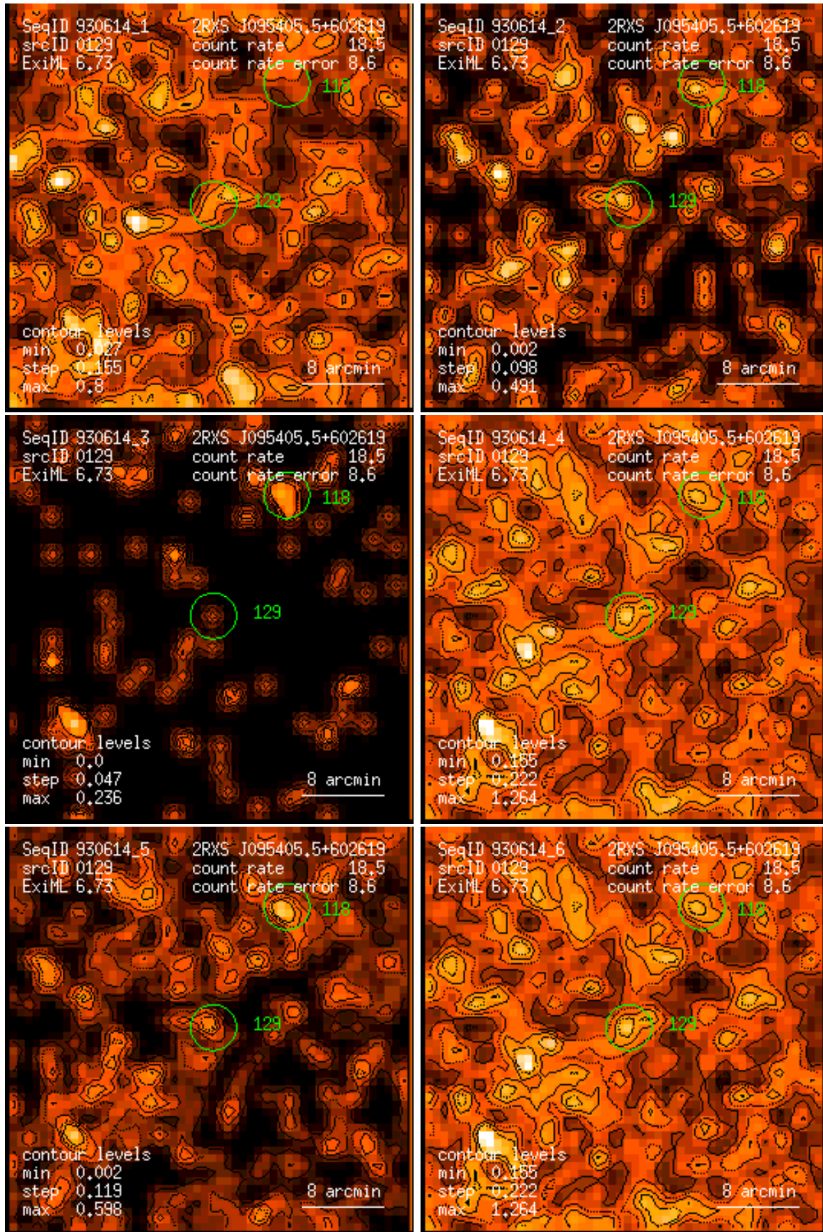
Figure 129: RASS 930614: detection 0129: band rate images, Gaussian filter: (1) PSPC channels 11 – 41, (2) 52 – 90, (3) 91 – 201, (4) 11 – 235, (5) 52 – 201, (6) 11 – 201. Broad band rates in counts/ks. Band rate contour levels in counts/ks/arcmin 2 .
