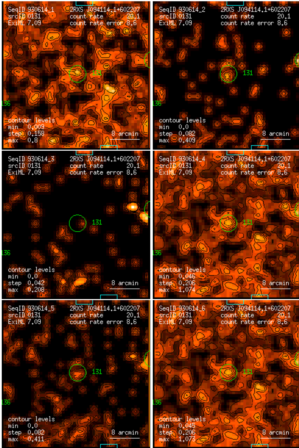
Figure 131: RASS 930614: detection 0131: band rate images, Gaussian filter: (1) PSPC channels 11 – 41, (2) 52 – 90, (3) 91 – 201, (4) 11 – 235, (5) 52 – 201, (6) 11 – 201. Broad band rates in counts/ks. Band rate contour levels in counts/ks/arcmin 2 .
