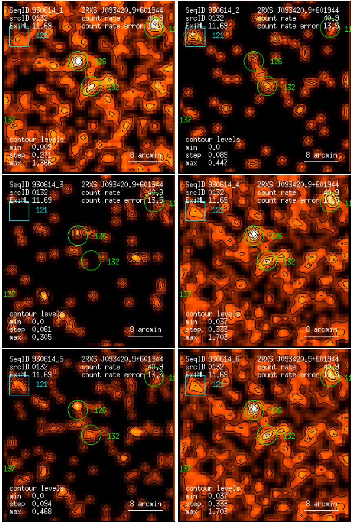
Figure 132: RASS 930614: detection 0132: band rate images, Gaussian filter: (1) PSPC channels 11 – 41, (2) 52 – 90, (3) 91 – 201, (4) 11 – 235, (5) 52 – 201, (6) 11 – 201. Broad band rates in counts/ks. Band rate contour levels in counts/ks/arcmin 2 .
