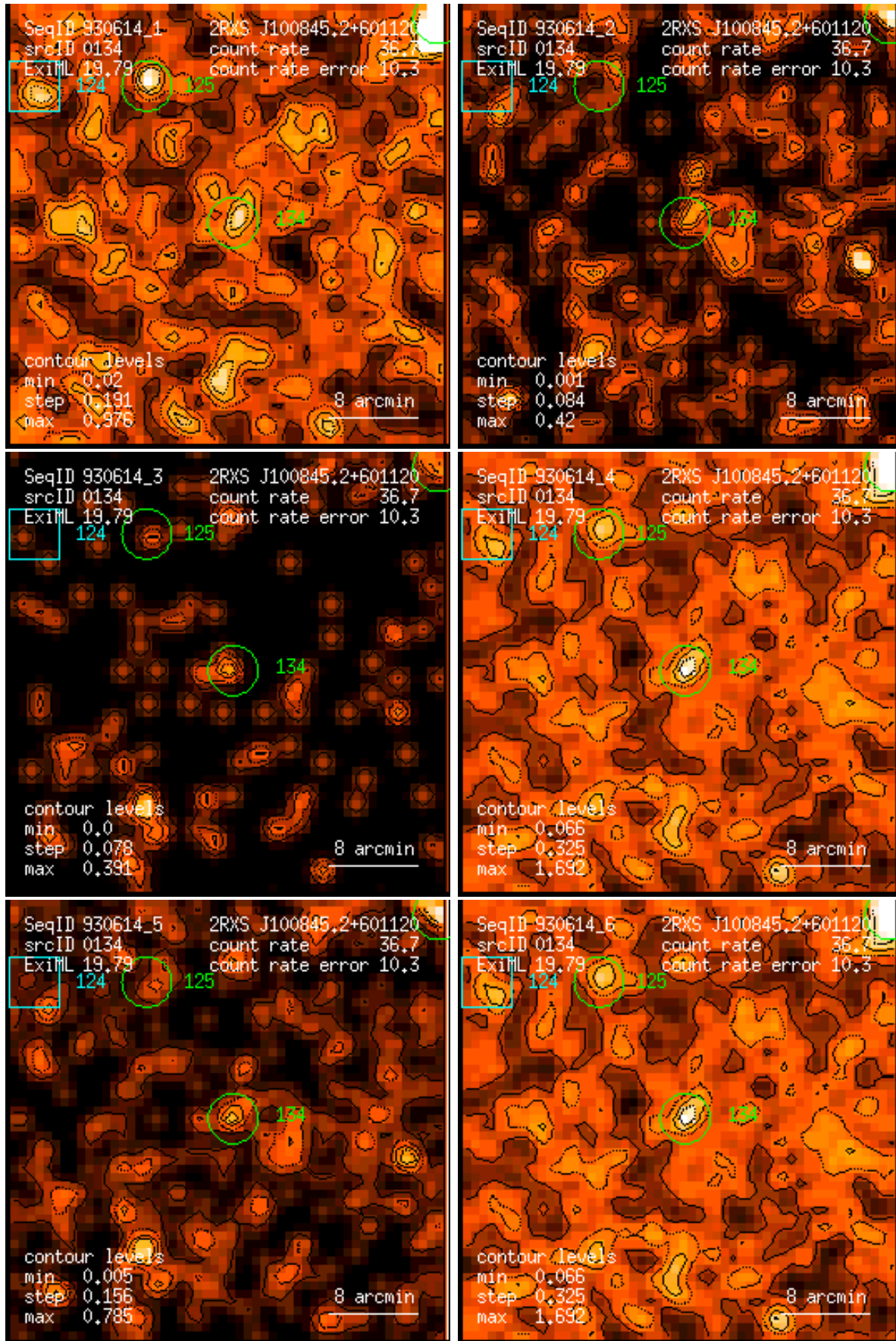
Figure 134: RASS 930614: detection 0134: band rate images, Gaussian filter: (1) PSPC channels 11 – 41, (2) 52 – 90, (3) 91 – 201, (4) 11 – 235, (5) 52 – 201, (6) 11 – 201. Broad band rates in counts/ks. Band rate contour levels in counts/ks/arcmin 2 .
