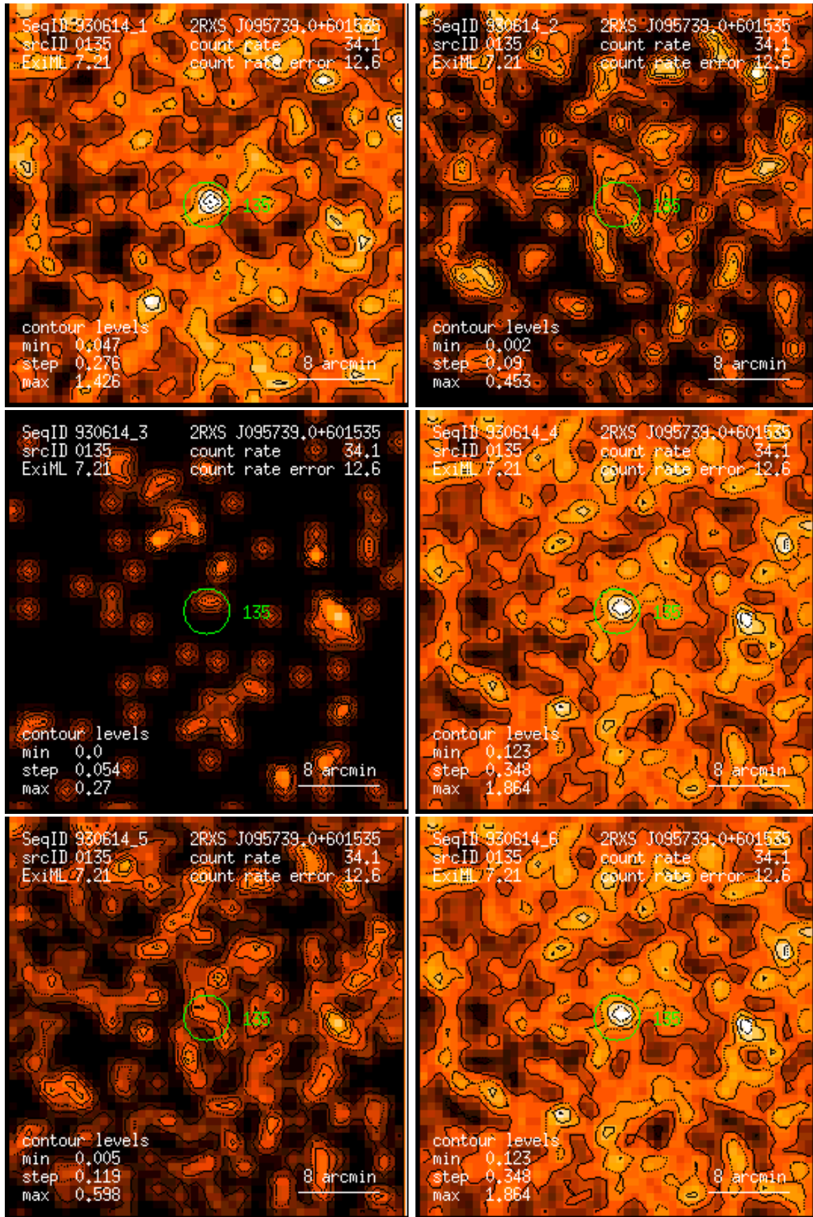
Figure 135: RASS 930614: detection 0135: band rate images, Gaussian filter: (1) PSPC channels 11 – 41, (2) 52 – 90, (3) 91 – 201, (4) 11 – 235, (5) 52 – 201, (6) 11 – 201. Broad band rates in counts/ks. Band rate contour levels in counts/ks/arcmin 2 .
