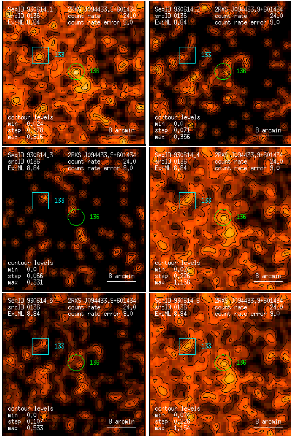
Figure 136: RASS 930614: detection 0136: band rate images, Gaussian filter: (1) PSPC channels 11 – 41, (2) 52 – 90, (3) 91 – 201, (4) 11 – 235, (5) 52 – 201, (6) 11 – 201. Broad band rates in counts/ks. Band rate contour levels in counts/ks/arcmin 2 .
