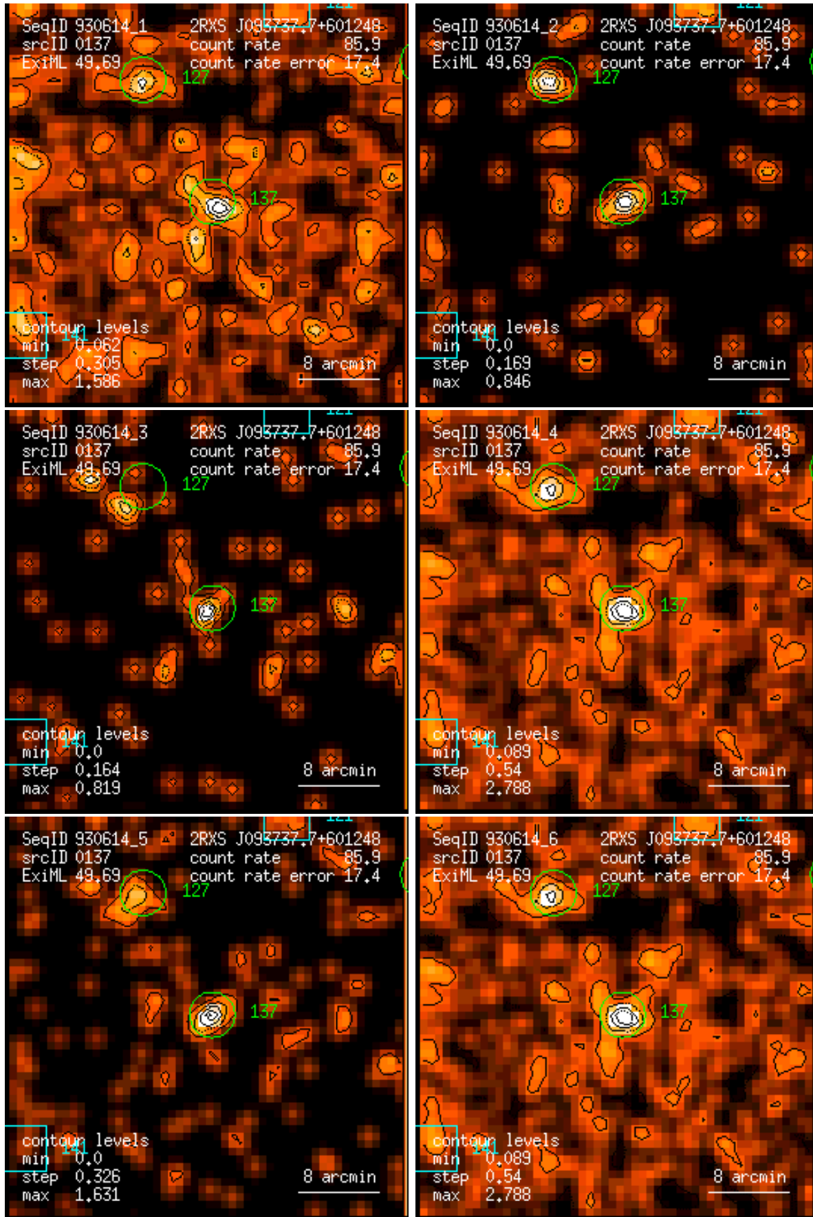
Figure 137: RASS 930614: detection 0137: band rate images, Gaussian filter: (1) PSPC channels 11 – 41, (2) 52 – 90, (3) 91 – 201, (4) 11 – 235, (5) 52 – 201, (6) 11 – 201. Broad band rates in counts/ks. Band rate contour levels in counts/ks/arcmin 2 .
