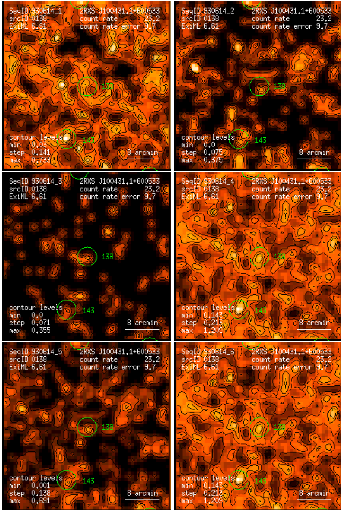
Figure 138: RASS 930614: detection 0138: band rate images, Gaussian filter: (1) PSPC channels 11 – 41, (2) 52 – 90, (3) 91 – 201, (4) 11 – 235, (5) 52 – 201, (6) 11 – 201. Broad band rates in counts/ks. Band rate contour levels in counts/ks/arcmin 2 .
