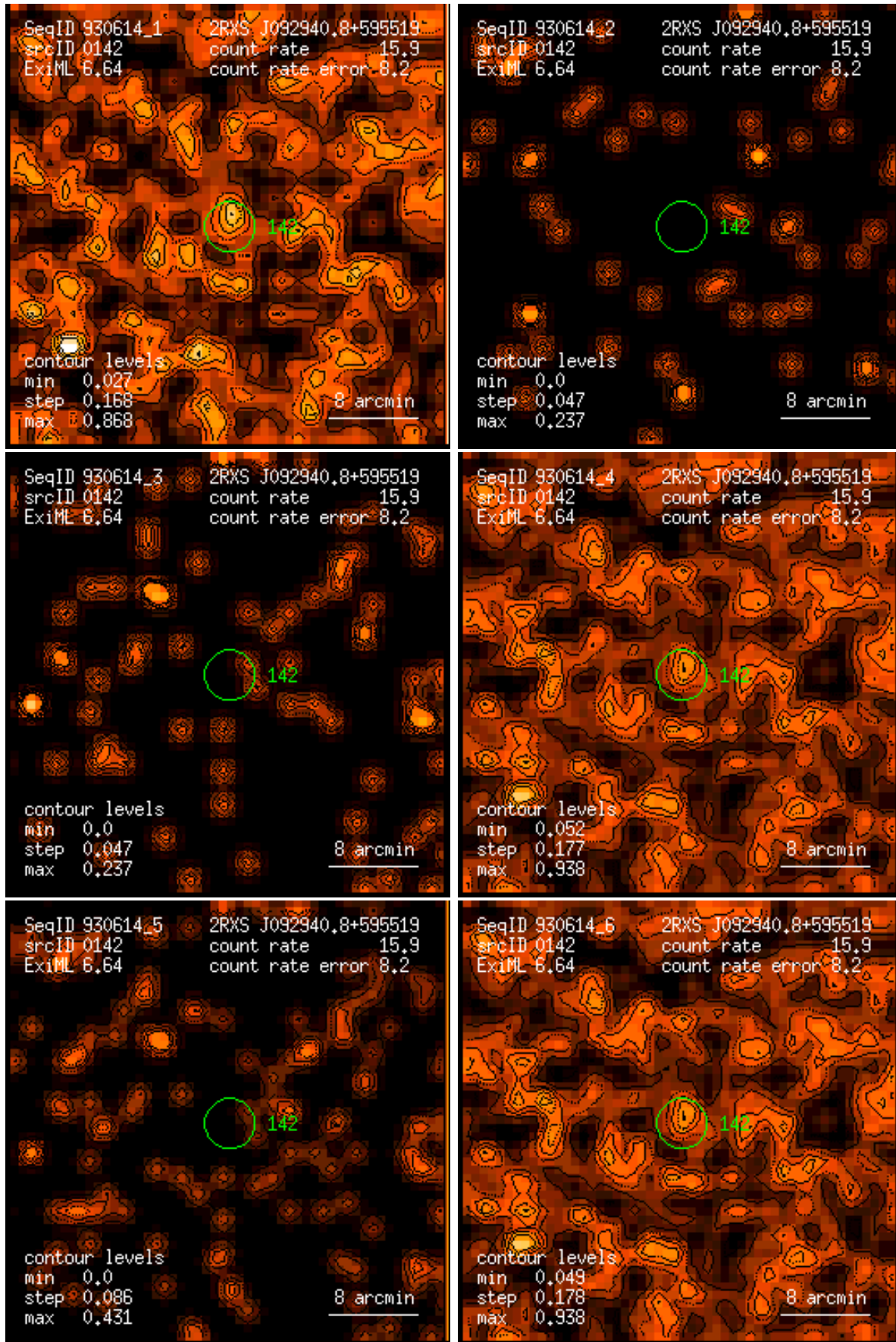
Figure 142: RASS 930614: detection 0142: band rate images, Gaussian filter: (1) PSPC channels 11 – 41, (2) 52 – 90, (3) 91 – 201, (4) 11 – 235, (5) 52 – 201, (6) 11 – 201. Broad band rates in counts/ks. Band rate contour levels in counts/ks/arcmin 2 .
