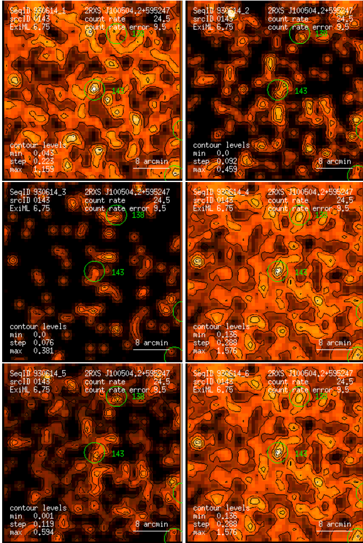
Figure 143: RASS 930614: detection 0143: band rate images, Gaussian filter: (1) PSPC channels 11 – 41, (2) 52 – 90, (3) 91 – 201, (4) 11 – 235, (5) 52 – 201, (6) 11 – 201. Broad band rates in counts/ks. Band rate contour levels in counts/ks/arcmin 2 .
