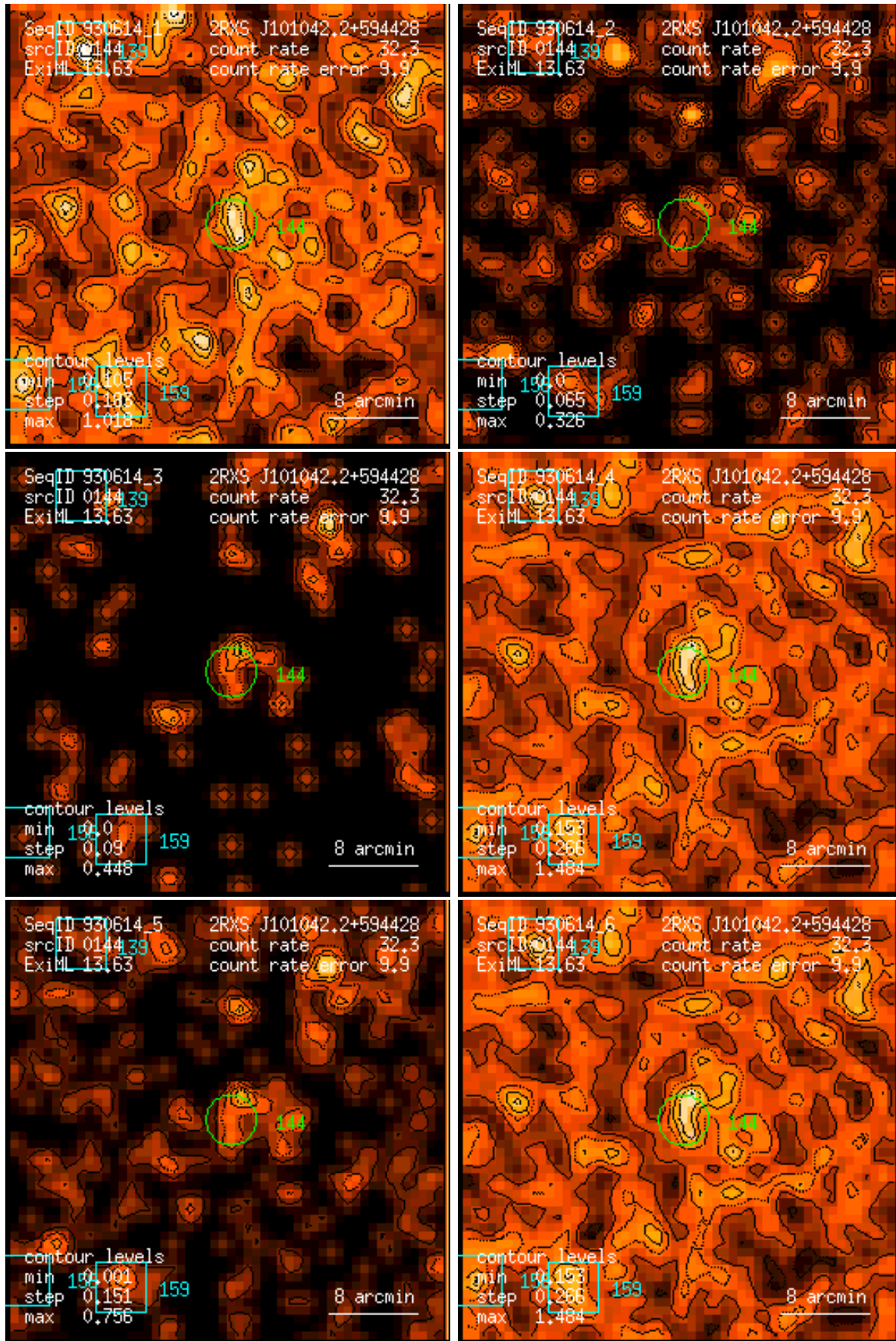
Figure 144: RASS 930614: detection 0144: band rate images, Gaussian filter: (1) PSPC channels 11 – 41, (2) 52 – 90, (3) 91 – 201, (4) 11 – 235, (5) 52 – 201, (6) 11 – 201. Broad band rates in counts/ks. Band rate contour levels in counts/ks/arcmin 2 .
