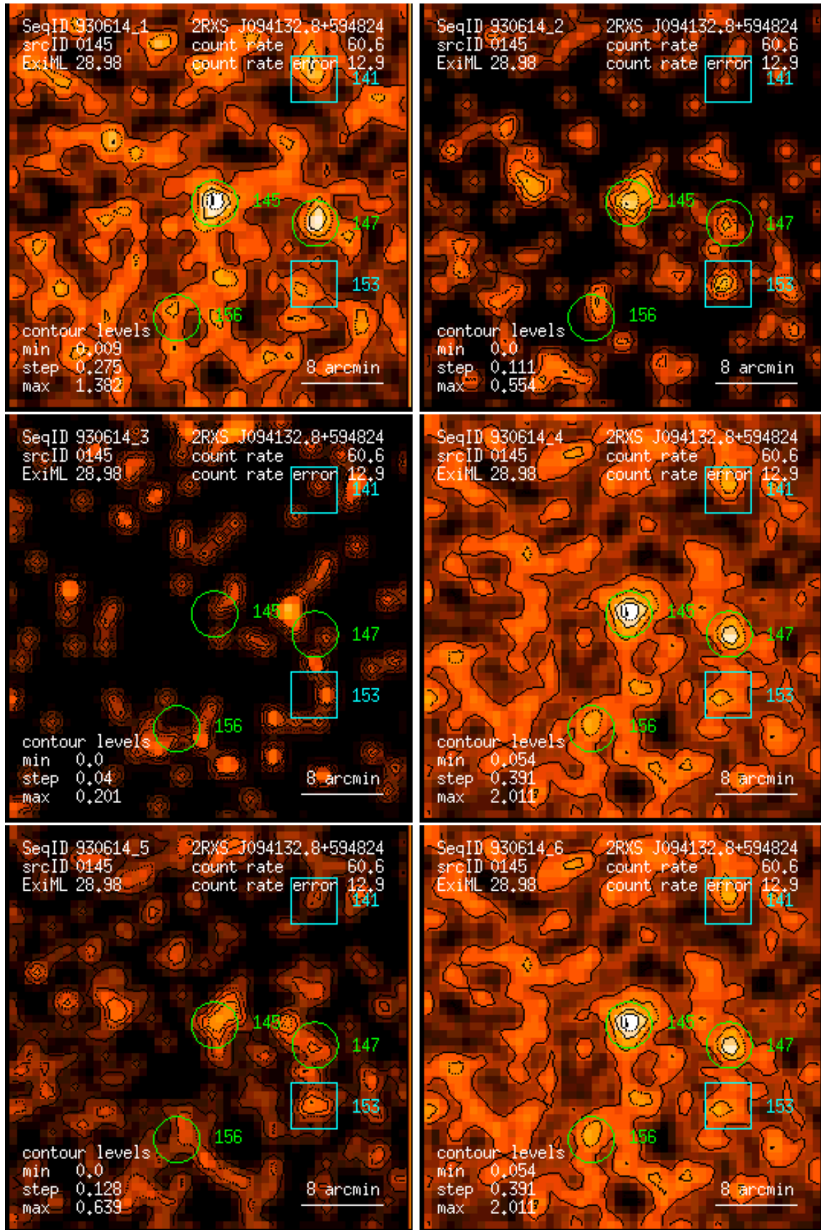
Figure 145: RASS 930614: detection 0145: band rate images, Gaussian filter: (1) PSPC channels 11 – 41, (2) 52 – 90, (3) 91 – 201, (4) 11 – 235, (5) 52 – 201, (6) 11 – 201. Broad band rates in counts/ks. Band rate contour levels in counts/ks/arcmin 2 .
