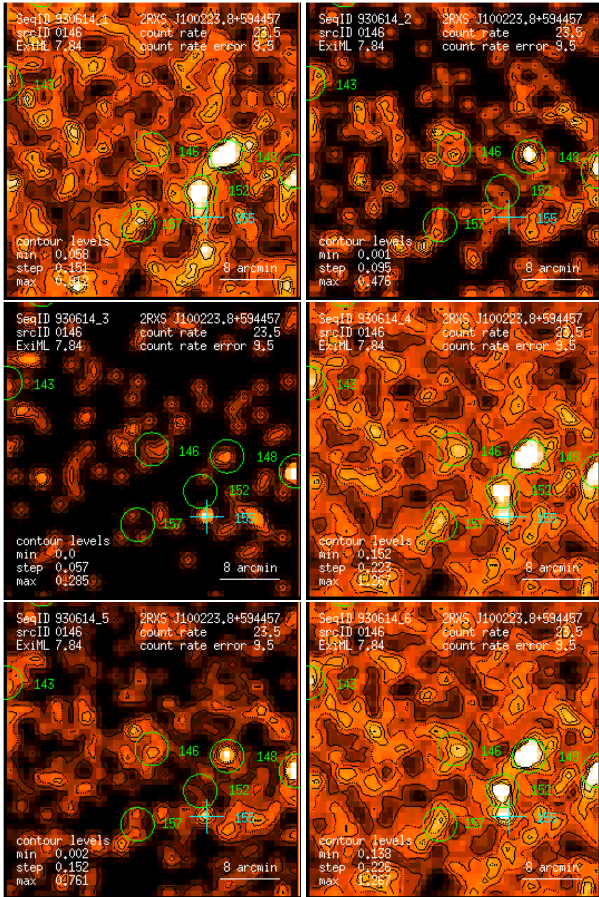
Figure 146: RASS 930614: detection 0146: band rate images, Gaussian filter: (1) PSPC channels 11 – 41, (2) 52 – 90, (3) 91 – 201, (4) 11 – 235, (5) 52 – 201, (6) 11 – 201. Broad band rates in counts/ks. Band rate contour levels in counts/ks/arcmin 2 .
