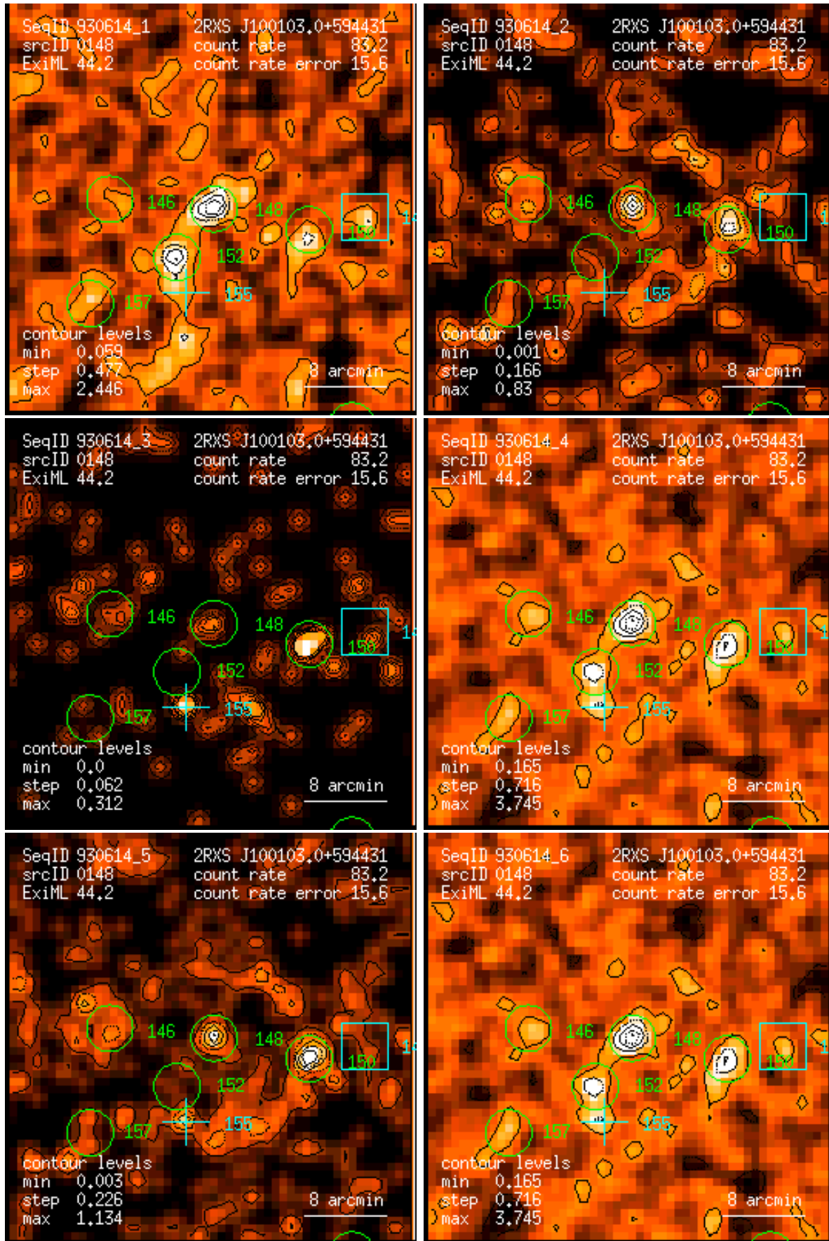
Figure 148: RASS 930614: detection 0148: band rate images, Gaussian filter: (1) PSPC channels 11 – 41, (2) 52 – 90, (3) 91 – 201, (4) 11 – 235, (5) 52 – 201, (6) 11 – 201. Broad band rates in counts/ks. Band rate contour levels in counts/ks/arcmin 2 .
