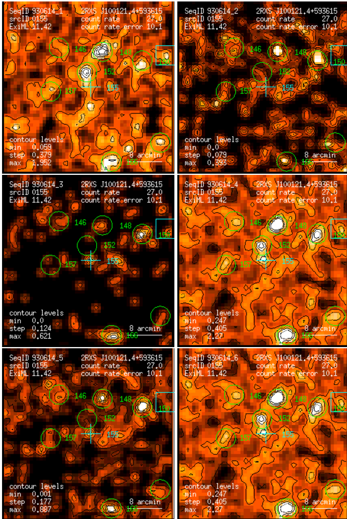
Figure 155: RASS 930614: detection 0155: band rate images, Gaussian filter: (1) PSPC channels 11 – 41, (2) 52 – 90, (3) 91 – 201, (4) 11 – 235, (5) 52 – 201, (6) 11 – 201. Broad band rates in counts/ks. Band rate contour levels in counts/ks/arcmin 2 .
