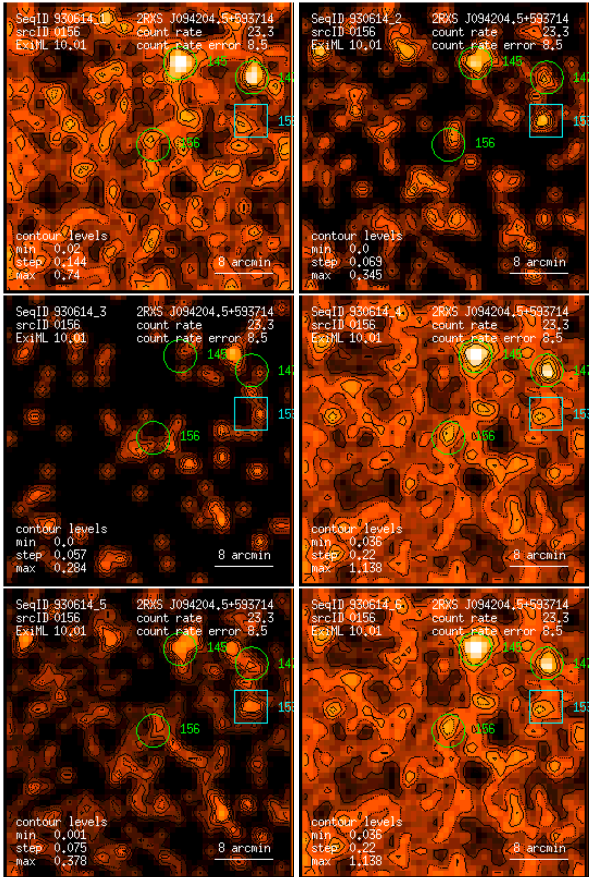
Figure 156: RASS 930614: detection 0156: band rate images, Gaussian filter: (1) PSPC channels 11 – 41, (2) 52 – 90, (3) 91 – 201, (4) 11 – 235, (5) 52 – 201, (6) 11 – 201. Broad band rates in counts/ks. Band rate contour levels in counts/ks/arcmin 2 .
