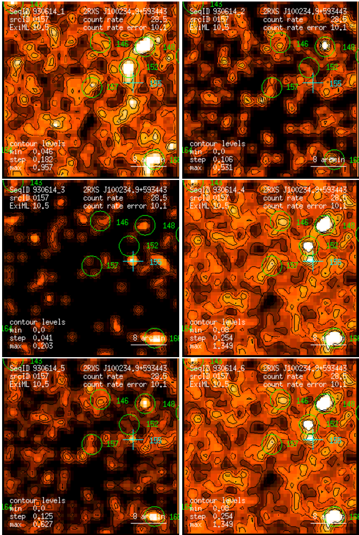
Figure 157: RASS 930614: detection 0157: band rate images, Gaussian filter: (1) PSPC channels 11 – 41, (2) 52 – 90, (3) 91 – 201, (4) 11 – 235, (5) 52 – 201, (6) 11 – 201. Broad band rates in counts/ks. Band rate contour levels in counts/ks/arcmin 2 .
