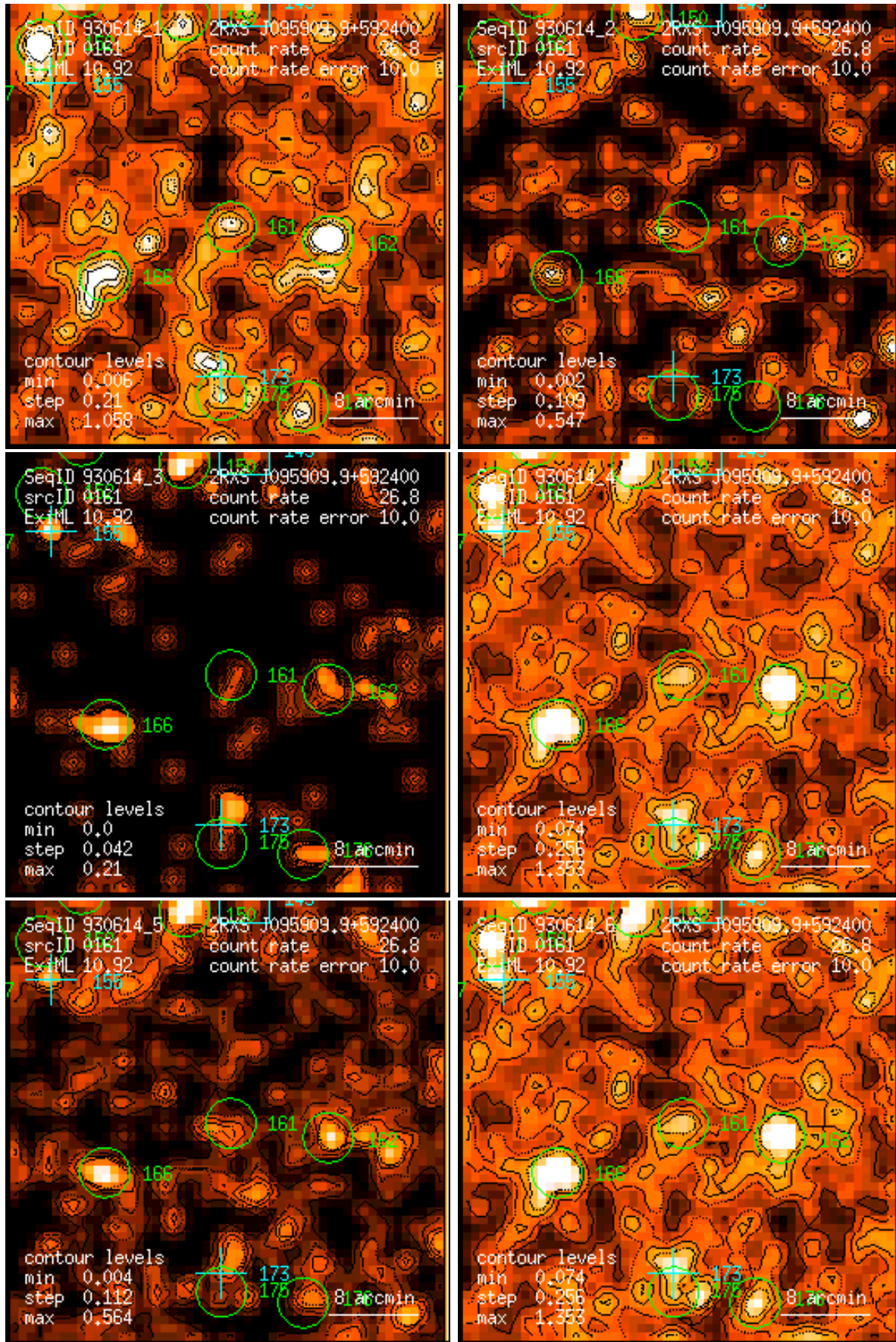
Figure 161: RASS 930614: detection 0161: band rate images, Gaussian filter: (1) PSPC channels 11 – 41, (2) 52 – 90, (3) 91 – 201, (4) 11 – 235, (5) 52 – 201, (6) 11 – 201. Broad band rates in counts/ks. Band rate contour levels in counts/ks/arcmin 2 .
