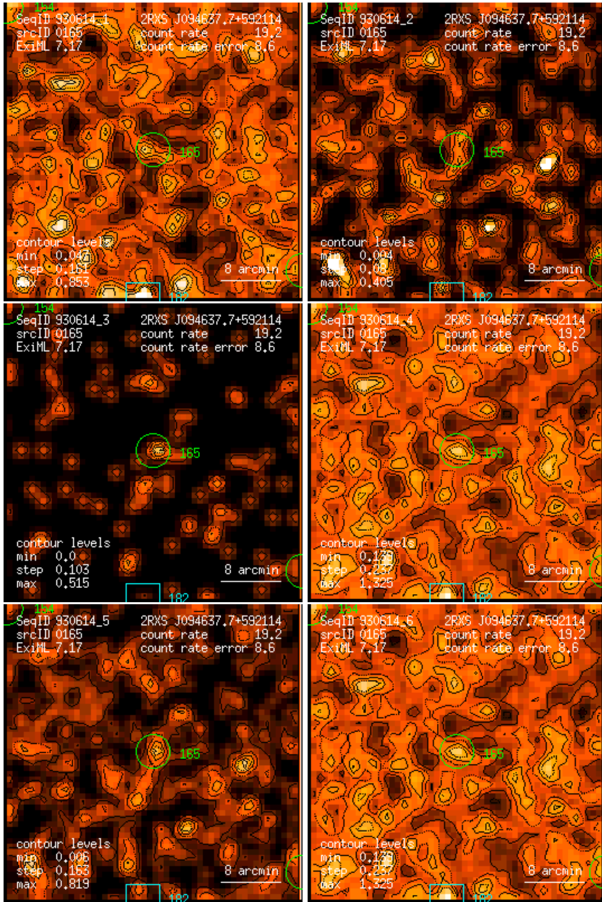
Figure 165: RASS 930614: detection 0165: band rate images, Gaussian filter: (1) PSPC channels 11 – 41, (2) 52 – 90, (3) 91 – 201, (4) 11 – 235, (5) 52 – 201, (6) 11 – 201. Broad band rates in counts/ks. Band rate contour levels in counts/ks/arcmin 2 .
