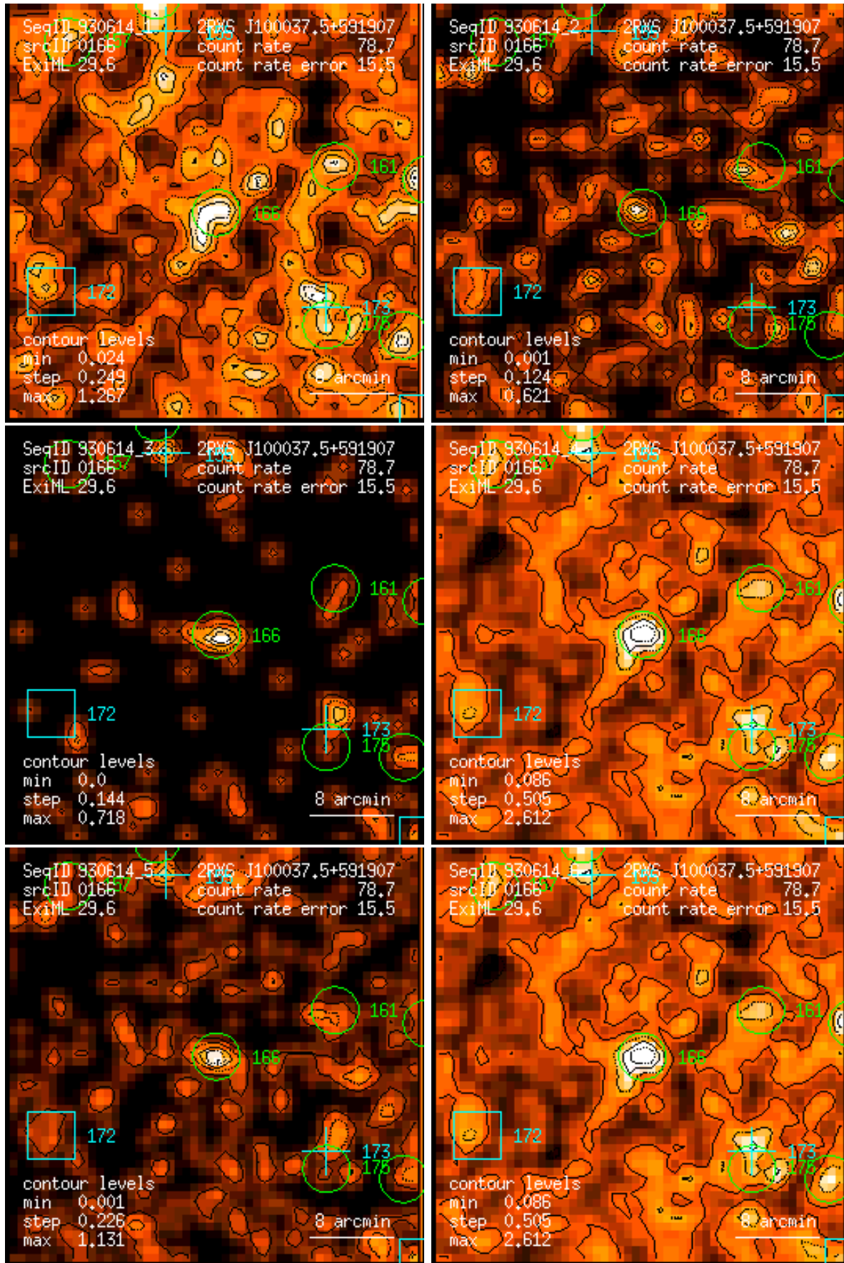
Figure 166: RASS 930614: detection 0166: band rate images, Gaussian filter: (1) PSPC channels 11 – 41, (2) 52 – 90, (3) 91 – 201, (4) 11 – 235, (5) 52 – 201, (6) 11 – 201. Broad band rates in counts/ks. Band rate contour levels in counts/ks/arcmin 2 .
