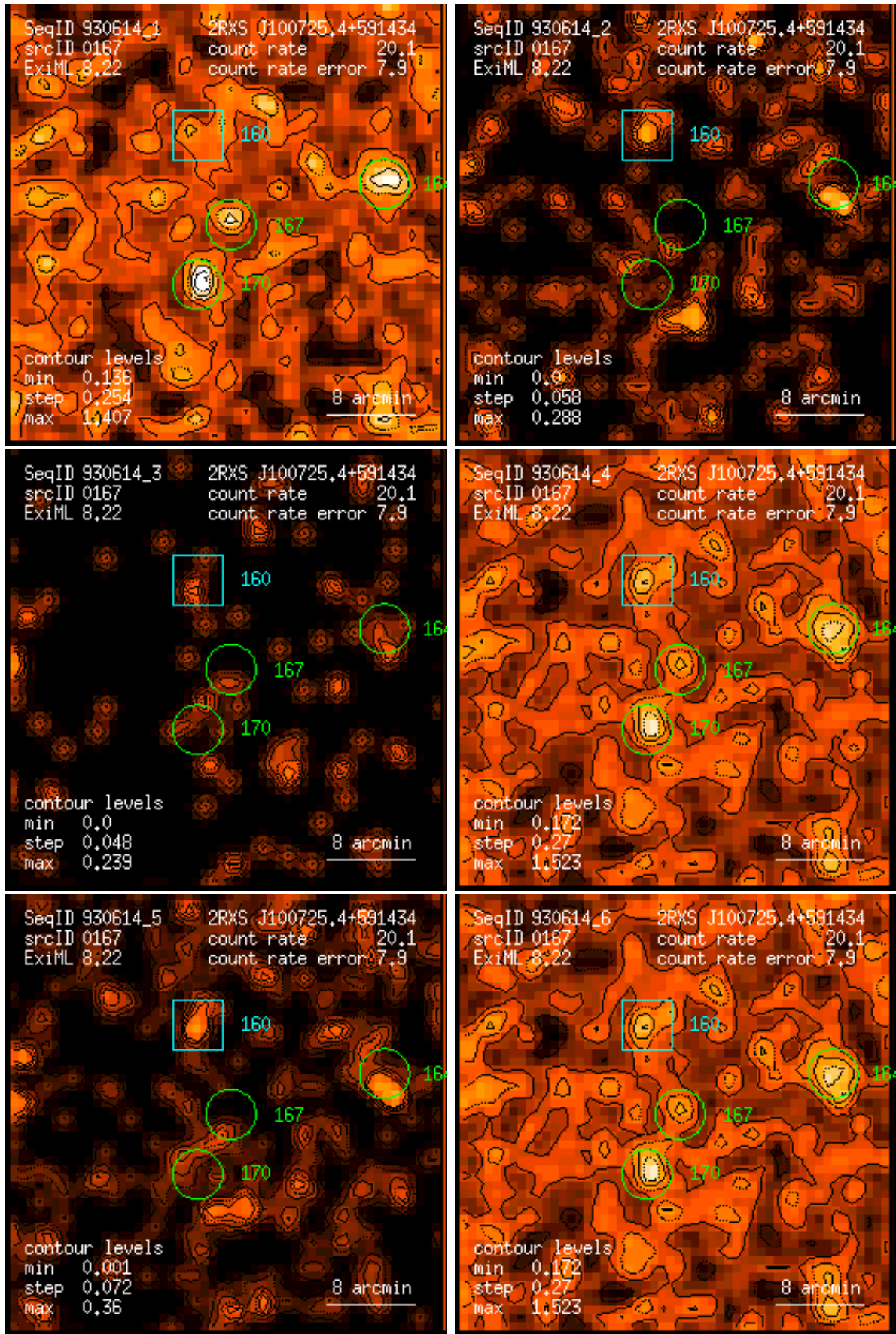
Figure 167: RASS 930614: detection 0167: band rate images, Gaussian filter: (1) PSPC channels 11 – 41, (2) 52 – 90, (3) 91 – 201, (4) 11 – 235, (5) 52 – 201, (6) 11 – 201. Broad band rates in counts/ks. Band rate contour levels in counts/ks/arcmin 2 .
