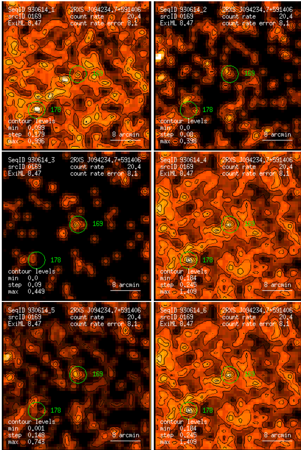
Figure 169: RASS 930614: detection 0169: band rate images, Gaussian filter: (1) PSPC channels 11 – 41, (2) 52 – 90, (3) 91 – 201, (4) 11 – 235, (5) 52 – 201, (6) 11 – 201. Broad band rates in counts/ks. Band rate contour levels in counts/ks/arcmin 2 .
