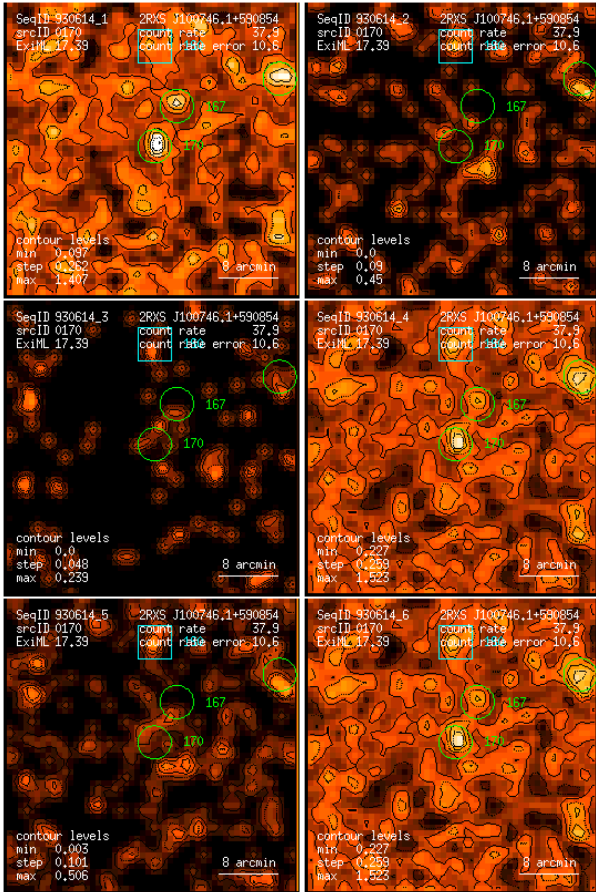
Figure 170: RASS 930614: detection 0170: band rate images, Gaussian filter: (1) PSPC channels 11 – 41, (2) 52 – 90, (3) 91 – 201, (4) 11 – 235, (5) 52 – 201, (6) 11 – 201. Broad band rates in counts/ks. Band rate contour levels in counts/ks/arcmin 2 .
