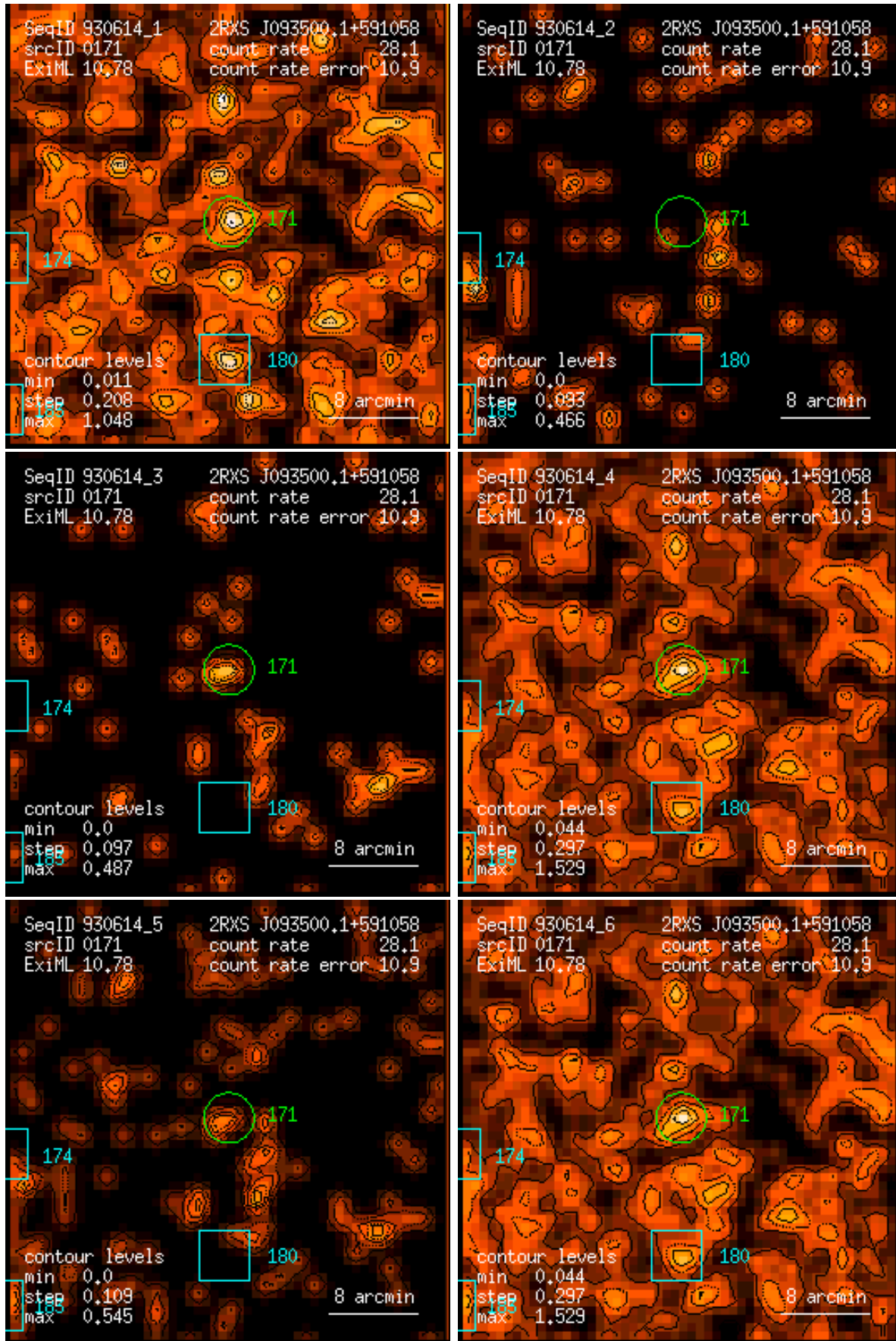
Figure 171: RASS 930614: detection 0171: band rate images, Gaussian filter: (1) PSPC channels 11 – 41, (2) 52 – 90, (3) 91 – 201, (4) 11 – 235, (5) 52 – 201, (6) 11 – 201. Broad band rates in counts/ks. Band rate contour levels in counts/ks/arcmin 2 .
